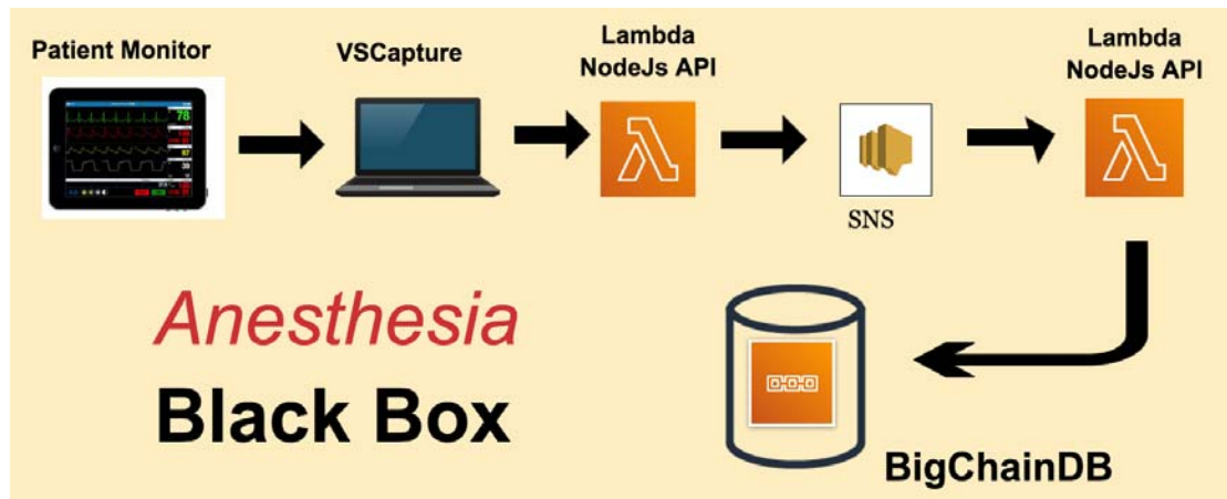
Figure 3: Data workflow.
