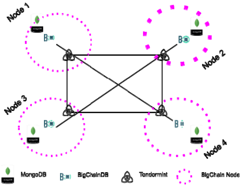
Figure 2: BigChainDB architecture.
