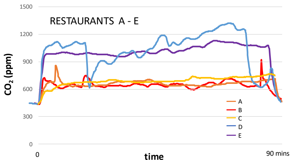
Figure 2: CO 2 concentration curves for the five restaurants sampled during the study. A, B and C record good, generally stable ventilation conditions, with average CO 2 <700ppm, in contrast to Restaurants D and E. Whereas Restaurant D made sporadic efforts to ventilate the establishment by opening the front door (marked by two precipitate falls towards 600ppm), Restaurant E kept doors and windows closed. See text for details.
