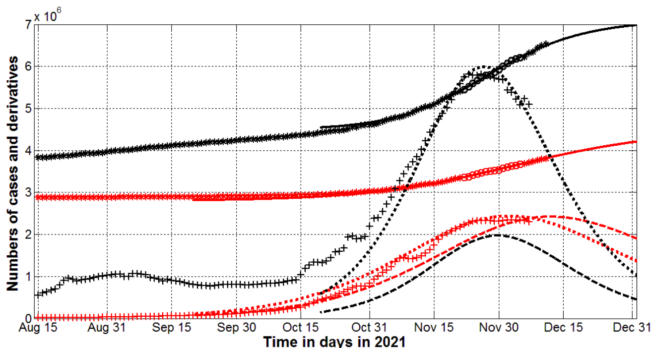
Figure. The COVID-19 pandemic waves in Poland (red) and Germany (black) in the autumn of 2021.
