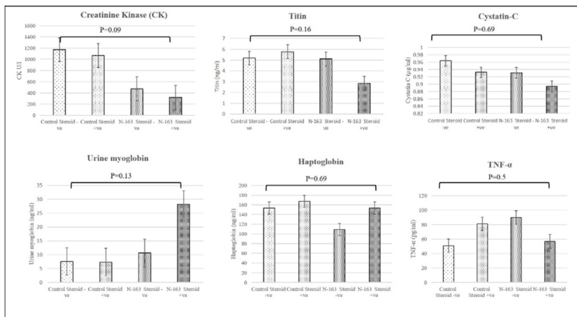
631 Figure 7: Levels of Creatinine kinase (CK), Titin, Cystatin-C, Urine myoglobin, Haptoglobin
