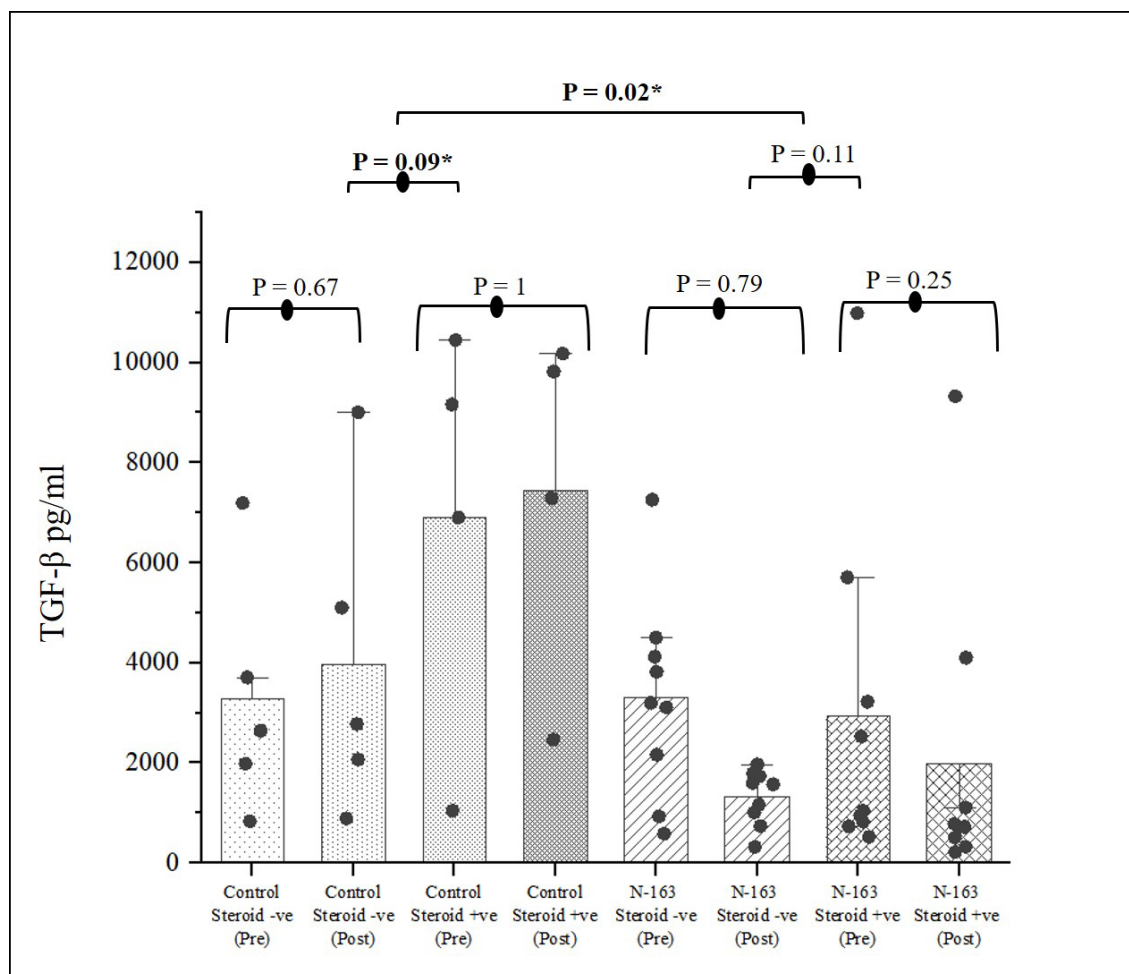
618 Figure 4: Levels of TGF-β showed significant decrease in the N-163 Steroid -ve group 619 compared to other groups (*p-value significance < 0.05)
