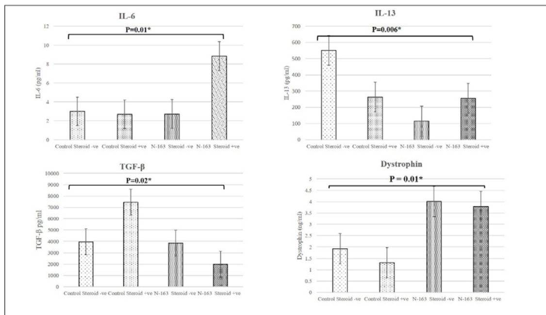
626 Figure 6: Comprehensive figure of IL-6, IL-13, TGF-β and Dystrophin showing comparison 627 of values between control and treatment group (N-163), pre- and post-intervention (*p-value 628 significance < 0.05)
