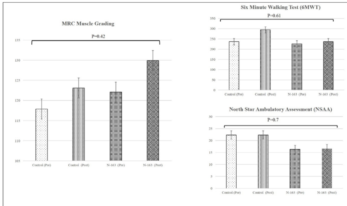
637 Figure 8: MRC muscle grading, 6MWT and NSAA results between control and treatment
