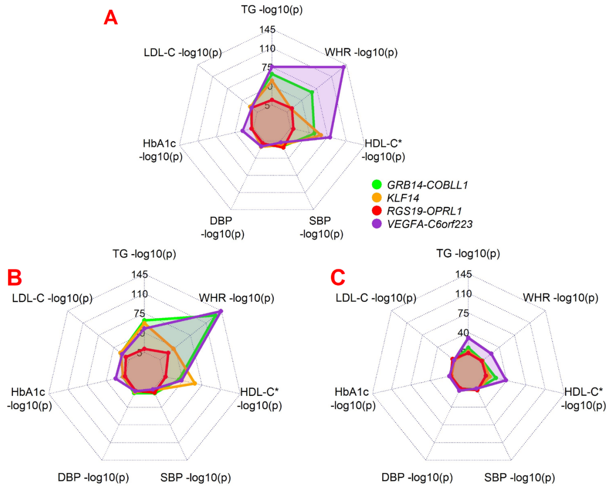
520 Figure 1: Radar plot showing association p-values for all four loci identified in UK Biobank in A) both men and women, B) women 521 only, and C) men only.
