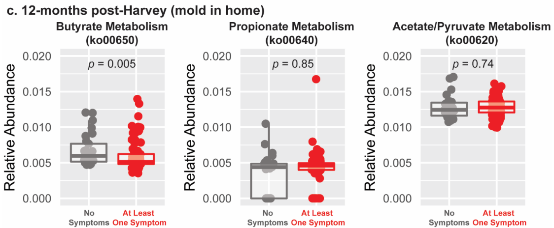
Figure 5. Relative abundance of bacterial genes involved in short-chain fatty acid (SCFA) metabolism in association with allergic symptoms. WGS sequencing was used to determine the relative abundance of metabolic pathways involved in the production of the three major SCFAs (butyrate, propionate, and acetate) at 1-month post-Harvey ( a , n=18 without symptoms, n=88 with symptoms), 12-months post-Harvey (all subjects) ( b , n=67 without symptoms, n=156 with symptoms) and 12-months post-Harvey (mold in home only) ( c , n=29 without symptoms, n=97 with symptoms). All statistical tests reported are one-sided Mann-Whitney tests. Box plots indicate median and interquartile range (IQR), whiskers show smallest (lower whisker) or largest (upper whisker) value within 1.5 times the IQR.
