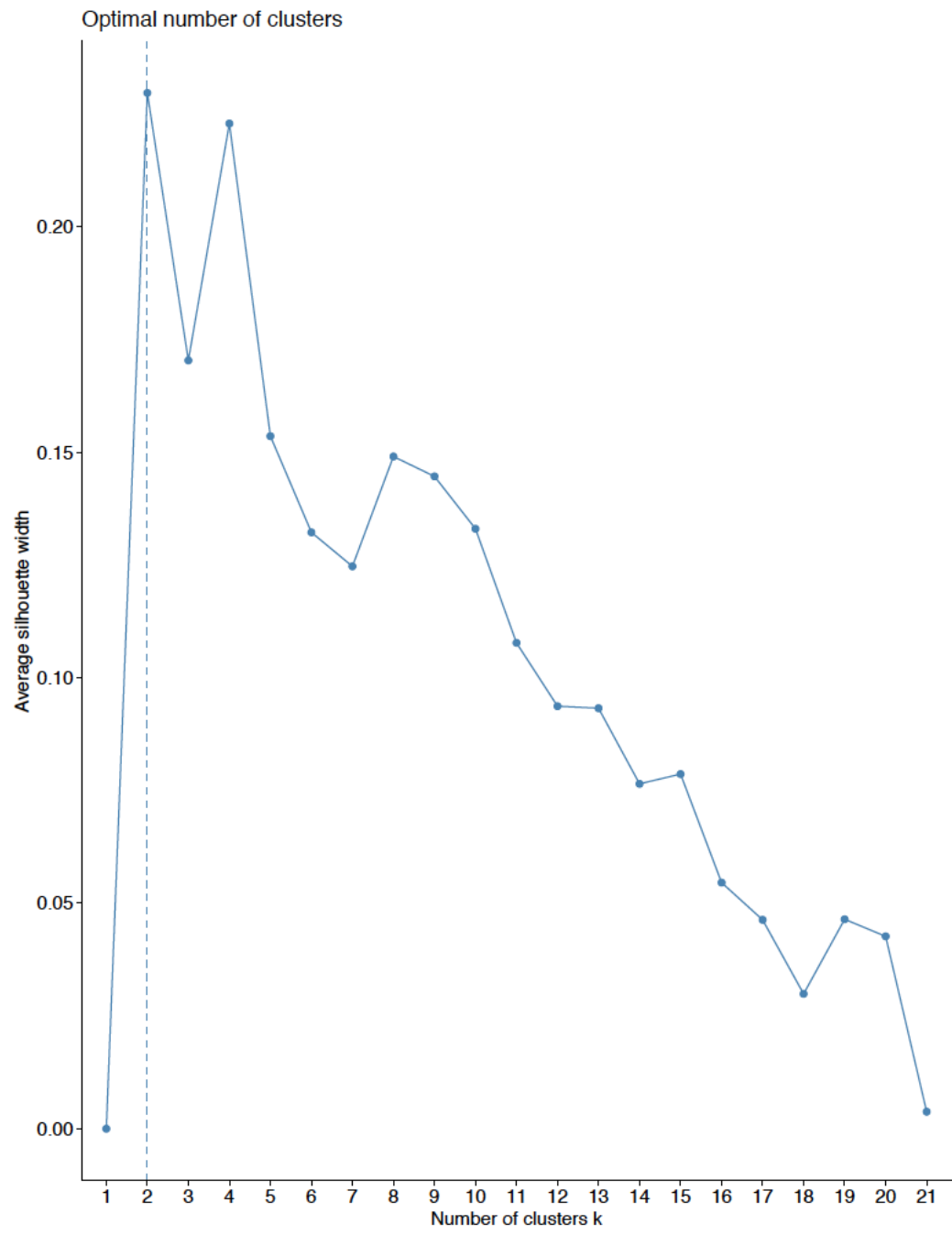
Figure 2. Silhouette Coefficients from K-Means Clustering Algorithm A silhouette coefficient determined that a 2-cluster solution was optimal to characterize the relationships between sleep/activity and substance use dimensions.
