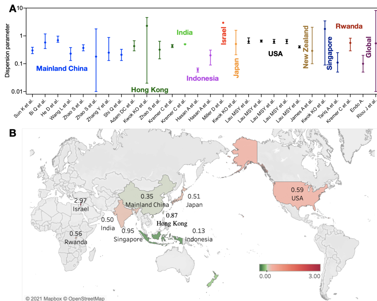
Figure 1. Dispersion parameter estimates for coronavirus disease 2019 (COVID-19) reported in 19 unique studies presented by country. (A) Estimates of dispersion parameters over countries. The error bars show the mean values and 95% confidence interval. (B) Mean estimate of dispersion parameters by countries over studies.
