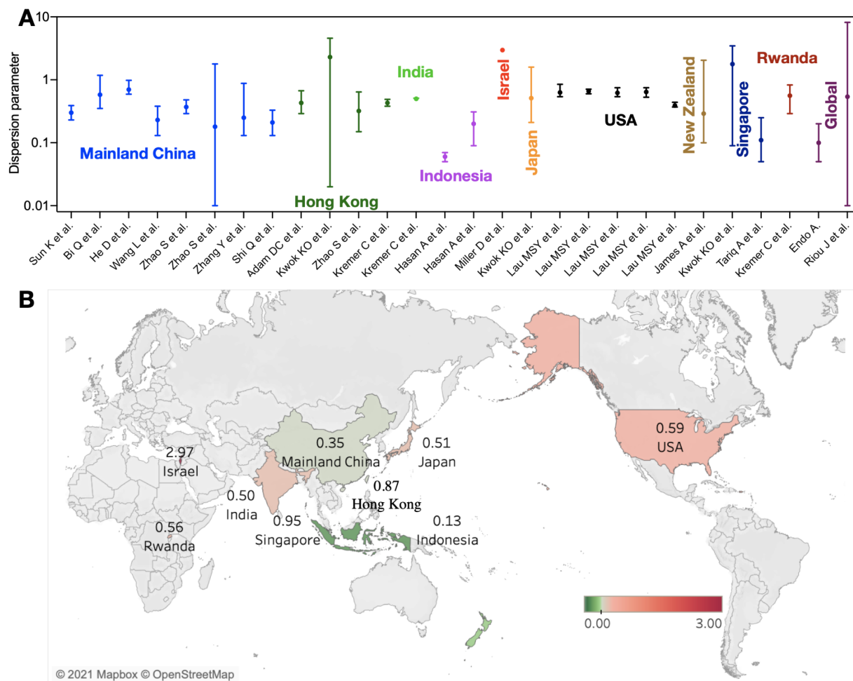
Figure 1. Dispersion parameter estimates for coronavirus disease 2019 (COVID-19) reported in 19 unique studies presented by country. (A) Estimates of dispersion parameters over countries. The error bars show the mean values and 95% confidence interval. (B) Mean estimate of dispersion parameters by countries over studies.
