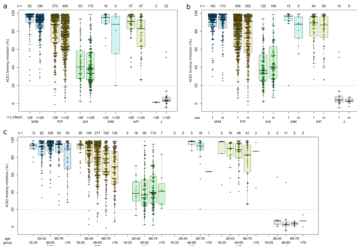
656 Fig. 4. Effect of time post-vaccination, gender and age on ACE2 binding inhibition for different SARS-CoV- 657 2 vaccination schemes.
