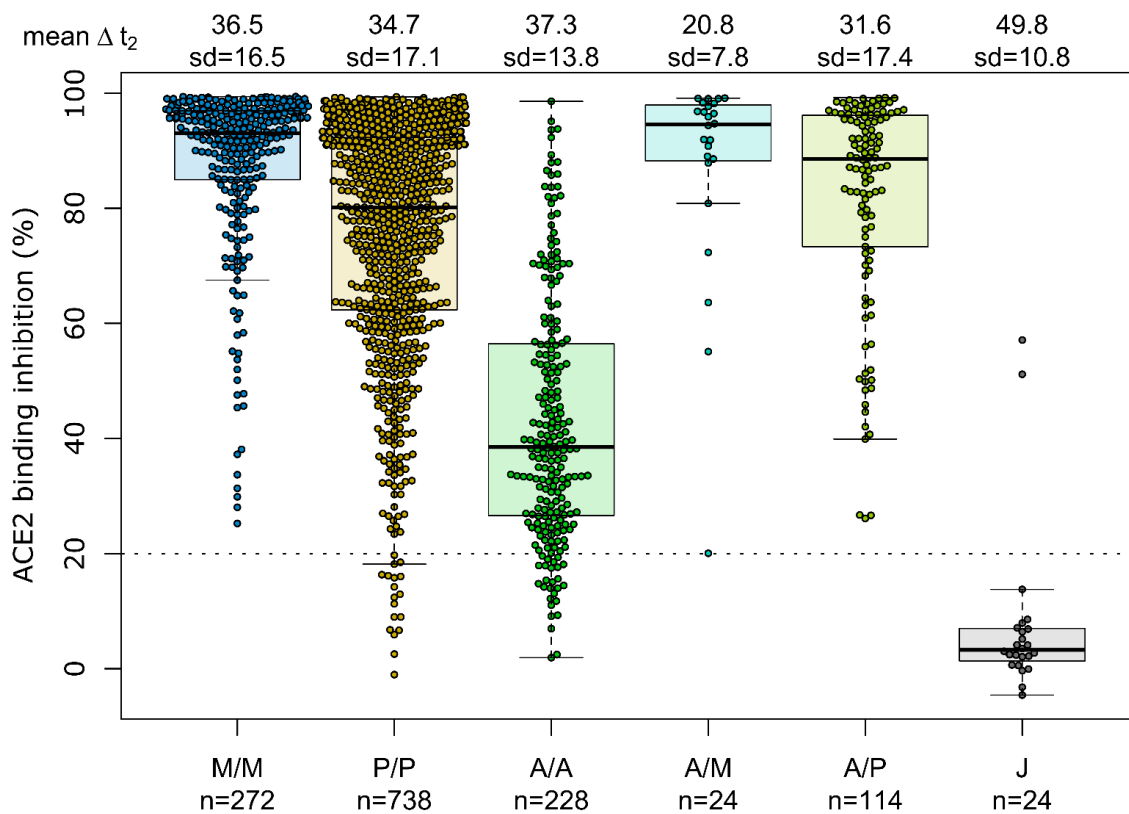
642 Fig. 3. Different vaccination schemes impact ACE2 binding inhibition against SARS-CoV-2 wild-type.
