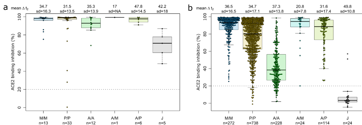
Fig. 5. SARS-CoV-2 vaccination boosts ACE2 binding inhibition among recovered individuals independent of vaccination scheme
