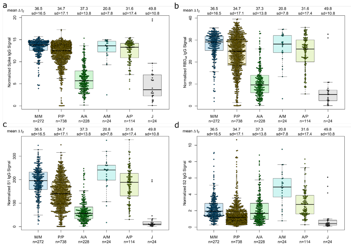
Fig. 1. Different SARS-CoV-2 vaccination schemes result in distinct humoral responses.
