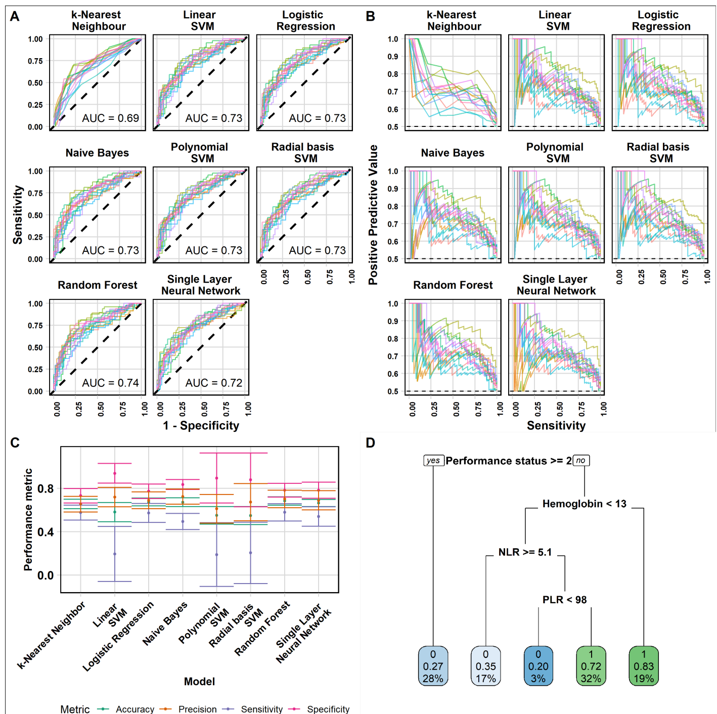
Figure 3: Machine learning algorithms predictive performances
