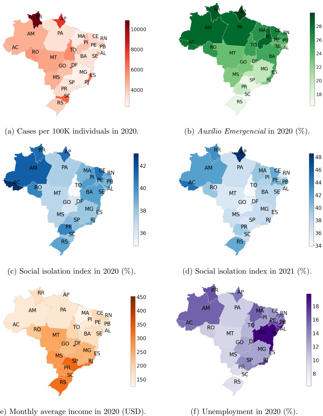
Figure 1: (a) Total number of COVID-19 infections per 100 thousand individuals for each state in Brazil during 2020. (b) Statewide median population proportions receiving the AE in 2020. Statewide median values of the social isolation index during 2020 (c) and 2021 (d). (e) Statewide monthly average income in 2020 (USD). (f) Statewide unemployment in 2020.
