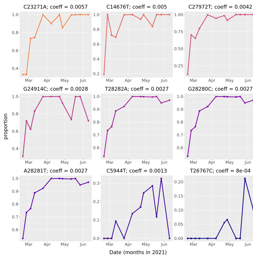
Figure 3: Mutations that significantly increase over time. The mutations were pooled over locations of 4 different wastewater treatment plants and daytime and sorted by decreasing coefficients from linear models. Statistical significance was evaluated by a t-test using p \leq 0.05 as cutoff. Only samples passing the sample quality scoring (> 90% mutation coverage) were used.
