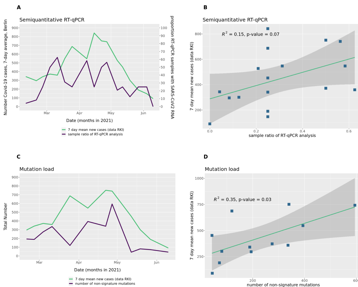
Figure 5: A) 7 days average of COVID-19 cases in Berlin, data from Robert Koch-Institute (RKI) (light green, left axis) and proportion of samples positively determined SARS-CoV-2 RNA by RT-qPCR (dark violet, right axis) over Feb - Jun 2021. B)
