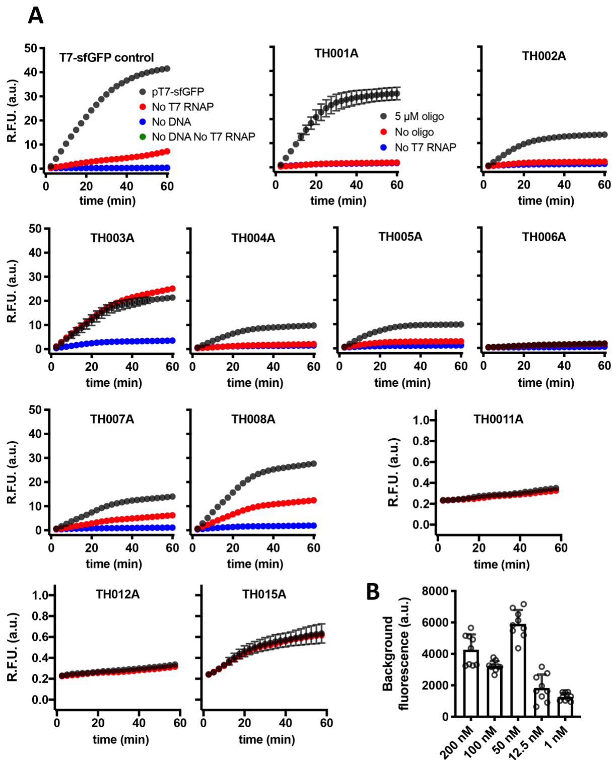
Figure S3. Functional screening of different toehold-switch-mediated riboregulatory elements. (A) Activities of different riboregulatory elements. (B) Minimum synthetic RNA concentrations that can activate gene expression in E. coli cell-free reaction. Note that 3' UTR toehold-switches did not succeed (TH011A, TH012A, TH015A), likely due to highly stable secondary structures of target RNAs.
