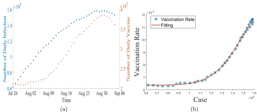
Figure 3: (a) Daily data on infections and vaccination rate from the Center for Disease Control (2021a). (b) The red solid line here represents the log-logistic function which estimates the vaccination rate.
