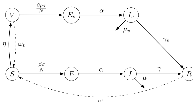
Figure 1: SEIR (Susceptible, Exposed, Infected, Recovered) type Compartmental Model. Here, people moves from susceptible ( S ) and vaccinated ( V ) compartment to exposed compartment ( E and E_v ) at \frac{\beta\sigma}{N} and \frac{\beta\rho\sigma}{N} respectively. From E and E_v people become infected ( I and I_v ) after incubation period \alpha . Then from I and I_v , infected people either go to the recovery compartment R or die. With the waning of antibodies, individuals move back to the S compartment from the R and V compartments.
