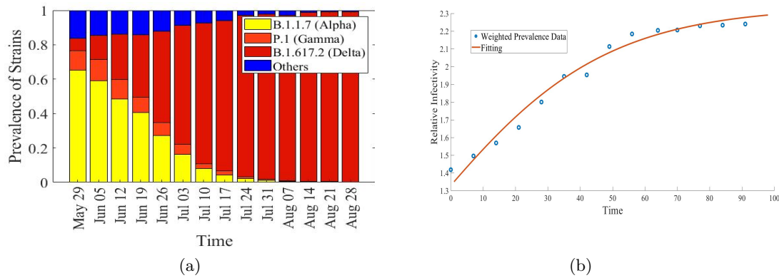
Figure 2: (a) Based on CDC’s Prevalence statistics, the change in prevalence of variants of coronavirus over time from May 29 to August 28 (Center for Disease Control, 2021a). (b) The relative infectivity of circulating viral variants is shown based on 50% increase in infectivity for alpha (B.1.1.7) with respect to other co-circulating variants and a 50% increase in infectivity for delta (B.1.617.2) in comparison to alpha (B.1.1.7) (blue circles). To estimate future relative infectivity, a log-logistic equation is fitted with the model (pink curve) (See Appendix B).
