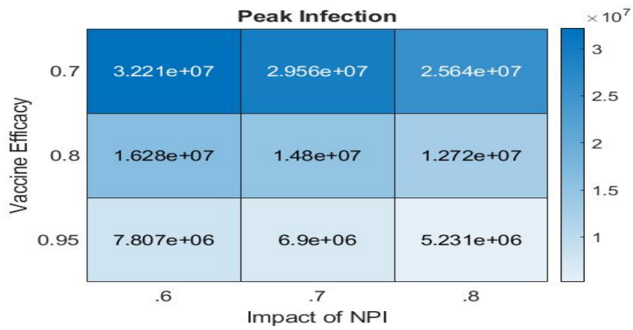
Figure 6: The variation in the peak value of daily infected cases as a function of NPI uptake and vaccination effectiveness. With an increase in NPI uptake or vaccine efficacy, the peak value is much lower.
