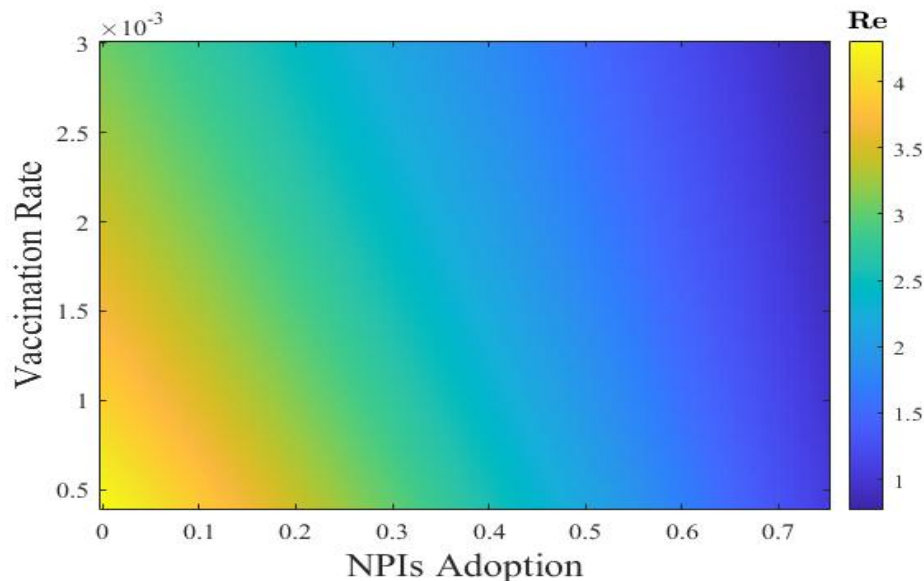
Figure 5: Heat-map here depicts how with fixed vaccine efficiency the effective reproduction number ( R_e ) varies with vaccination rates and adoption of NPIs. With vaccine efficacy 80%, the most efficient method to halt the spread of the disease is to increase immunization rates paired with good implementation of NPIs until herd immunity is reached.
