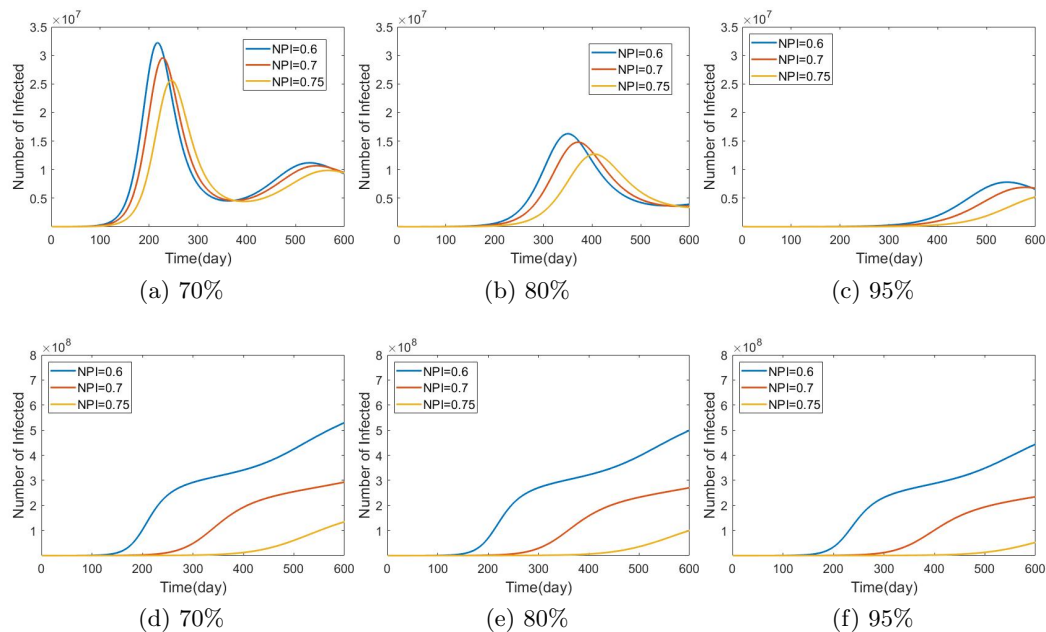
Figure 4: The effect of NPIs adoption and vaccine efficacy on the daily number of infected cases is depicted in this figure. Figures a, b, and c depict the change in daily case count with fixed vaccine efficacy (70%, 80%, 95%) with changing adoption of NPIs, while figures d, e, and f depict the corresponding cumulative case count. From a, b, c, d, e, f it is clear that if the majority of the population uses NPIs, NPIs will have the greatest influence on lowering the daily number of instances in the short and long term. If NPI adoption is not achievable, the only way to minimize the number of cases is to have a high vaccination rate with high effectiveness. (Check out Appendix C for a comparison of peak values.)
