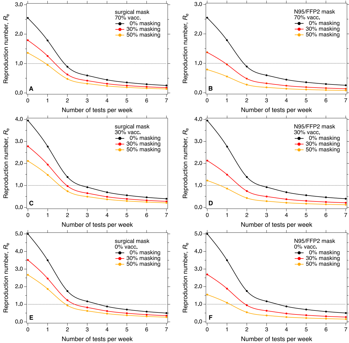
Fig. S7 Effectiveness of testing & isolation for different compliances with masking, vaccination, and distancing & ventilation. The same as Fig. 5, but with varies of combination of vaccination rates (“vacc.”), compliance of universal masking (“masking”) and distancing & ventilation (“dist. & vent.”). Reduction of effective reproduction number, R_e , as a function of testing frequency (number tests per week per person) for different compliances with universal masking and distancing & ventilation, as well as different vaccination rates. Basic reproduction number R_0 = 5 ; reduced starting values of R_e reflect different vaccination rates and compliances with masking and with distancing & ventilation, respectively. Left column corresponds to universal masking with surgical masks, right column corresponds to N95/FFP2 masks.
