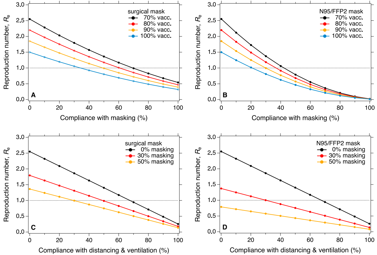
Fig. 2 Effectiveness of masking and distancing & ventilation for different vaccination rates and compliances. Reduction of effective reproduction number, R_e , as a function of compliance with universal masking for different vaccination rates (A, B) and as a function of compliance with distancing & ventilation for different levels of masking at a fixed vaccination rate of 70% (C, D). Basic reproduction number R_0 = 5 ; reduced starting values of R_e at zero compliance with masking correspond to different vaccination rates. Left column corresponds to universal masking with surgical masks, right column corresponds to N95/FFP2 masks.
