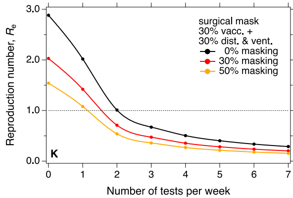
Fig. S7 (Continued)
