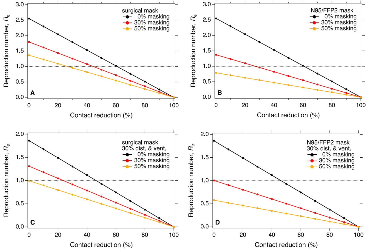
Fig. 3 Effectiveness of contact reduction for different compliances with masking and distancing & ventilation. Reduction of effective reproduction number, R_e , as a function of contact reduction for different compliances with universal masking at a fixed vaccination rate of 70%. Basic reproduction number R_0 = 5 ; reduced starting values of R_e at zero contact reduction reflect the vaccination rate and different levels of masking and distancing & ventilation (30% compliance, panels C and D). Left column corresponds to universal masking with surgical masks, right column corresponds to N95/FFP2 masks.
