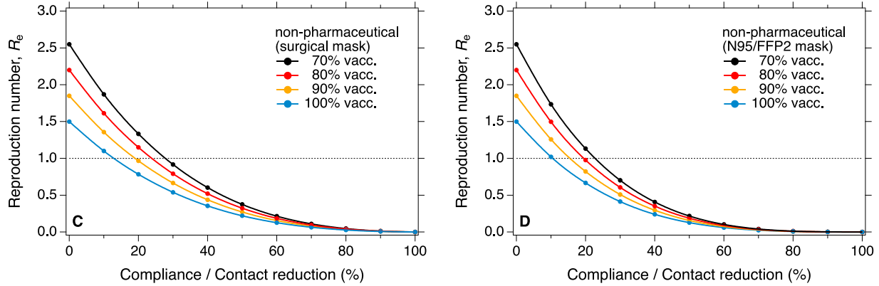
Fig. S6 Effectiveness of non-pharmaceutical measures for different vaccination rates. Reduction of effective reproduction number, R_e , as a function of compliance with non-pharmaceutical measures for different vaccination rates in the population. Non-pharmaceutical measures are the combination and synergy of universal masking, distancing and ventilation and contact reduction. Basic reproduction number R_0 = 5 ; reduced starting values of R_e at zero compliance with non-pharmaceutical measures correspond to different vaccination rates. Panels A and B refer to universal masking with surgical masks and N95/FFP2 masks, respectively.
