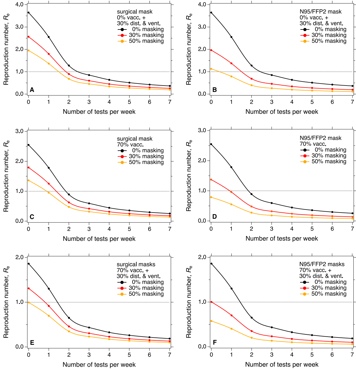
Fig. 4 Effectiveness of testing & isolation for different compliances with masking, vaccination, and distancing & ventilation. Reduction of effective reproduction number, R_e , as a function of testing frequency (number tests per week per person) for different compliances with universal masking and distancing & ventilation, as well as different vaccination rates. Basic reproduction number R_0 = 5 ; reduced starting values of R_e reflect different vaccination rates and compliances with masking and with distancing & ventilation, respectively. Left column corresponds to universal masking with surgical masks, right column corresponds to N95/FFP2 masks.
