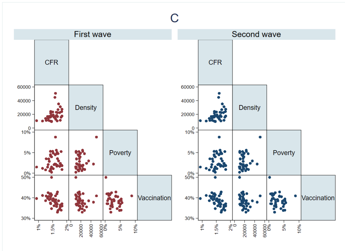
Fig. 3 Overall case fatality rate (CFR) by sub-district (A), age-specific CFR per sub-district and by pandemic wave (B), and correlation between CFR with sub-district population density, poverty, and COVID-19 vaccine coverage by epidemic wave (C).
