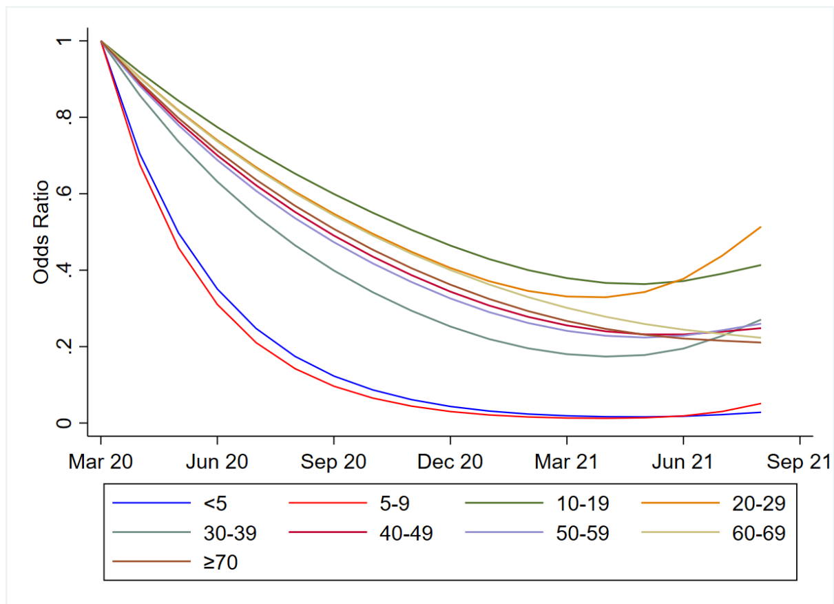
Fig. 4 Final multi-level logistic regression model showing individual, community, and health care factors associated with COVID-19 mortality (A), and age-specific COVID-19 mortality risk over time (B) in DKI Jakarta, Indonesia, March 2, 2020 to August 31, 2021. Sub-district was treated as the random effect variable in both models. For analysis presented in Figure A, first wave=March 2020 to April 2021. Second wave=May 2021 to August 2021. Numeric values were categorised into quartiles (Q), i.e., below 25 th percentile (Lowest), 25 th –50 th percentile (Q2), 50 th –75 th percentile (Q3) and above 75 th percentile (Highest) for each sub-district level variable. For Figure B, each line represents age-specific odds ratio estimates obtained from restricted cubic spline multi-level logistic regression model.
