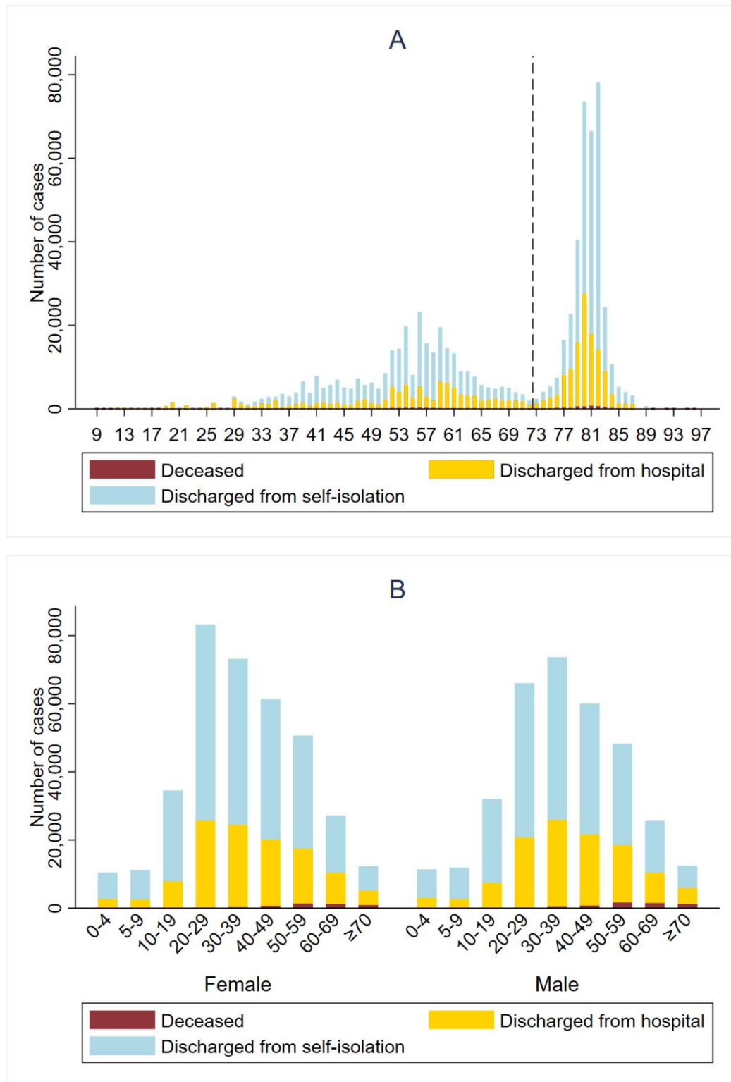
Figure S1. Outcomes over time (A), over age and by gender (B). Dashed black line represents the cut-off between the first and the second wave.
