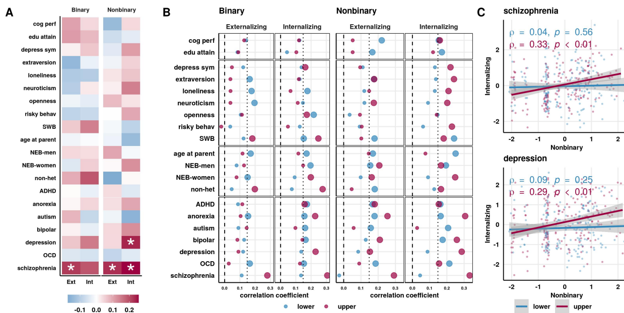
Figure 4. Correlations and interactions between gender diversity, mental health, and polygenic scores
