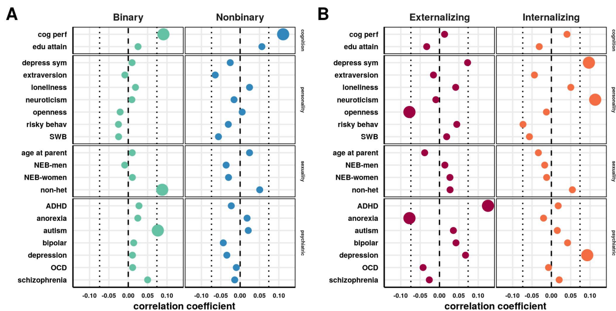
Figure 3. Polygenic score correlations with gender diversity and mental health
