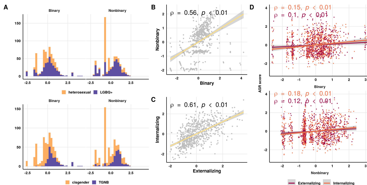
Figure 2. Distributions and correlations of the gender diversity and mental health measures
