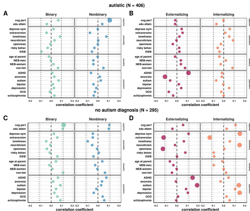
Figure S1. Polygenic score correlations with gender diversity and mental health separated by autism diagnostic status.
