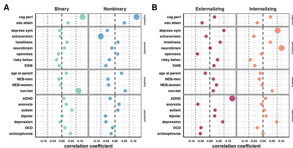
Figure S2. Polygenic score correlations with gender diversity and mental health in the Europe genetic ancestry population only ( N = 644 ).
