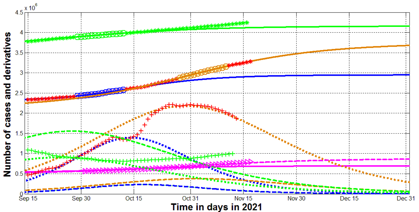
Fig. 2. The COVID-19 pandemic waves in Ukraine and in the whole world in the autumn of 2021. The results of SIR simulations of the 12th and 13th waves in Ukraine are shown by blue and brown lines, respectively. Green lines represent the 6th pandemic wave in the whole world. Numbers of victims V(t)=I(t)+R(t) – solid lines (for the world divided by 60); numbers of infected and spreading I(t) (multiplied by 5 for Ukraine) – dashed; derivatives dV/dt (eq. (2), multiplied by 100 for Ukraine and by 2 for the world) – dotted. The magenta lines represent the estimation of the accumulated number of deaths during the 12th (solid) and 13th (dashed) epidemic waves in Ukraine multiplied by 10. Magenta “triangles” represent the accumulated numbers of death in Ukraine from Table 1 multiplied by 10. “Circles” correspond to the accumulated numbers of cases registered during the periods of time taken for SIR simulations (for the world divided by 60). “Stars” corresponds to V_j values beyond these time periods (for the world divided by 60). “Crosses” show the first derivative (4) multiplied by 100 for Ukraine and by 2 for the world.
