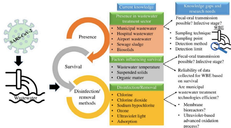
FIGURE 2. Features of SARS-CoV-2 in wastewater [39].
