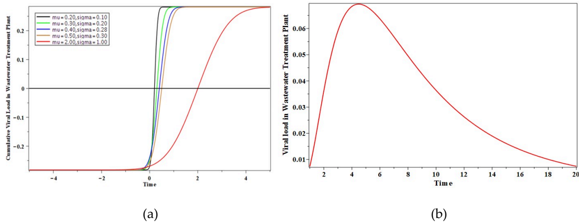
FIGURE 5. Gaussian model (a) predicting the possible cumulative SARS-CoV-2 load in WWTP, (b) predicting the possible SARS-CoV-2 load in WWTP.
