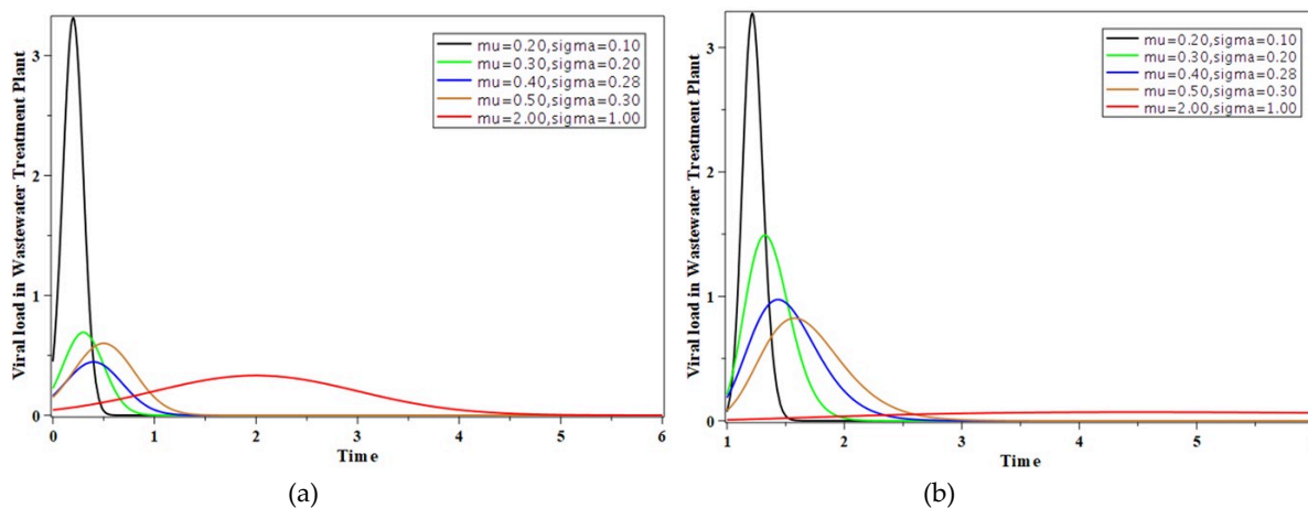
FIGURE 4. (a) Possible SARS-CoV-2 load in WWTP using Normal model, and (b) Possible SARS-CoV-2 load in WWTP using Log Normal model.
