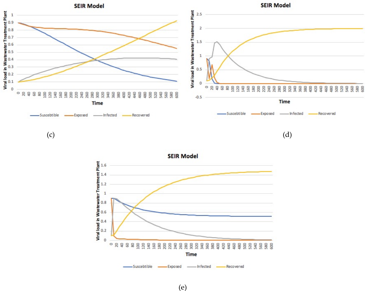
FIGURE 6. Numerical solution for SEIR mode with (a) \beta = 0.0095 , \gamma = 0.004 , \sigma = 0.01 , (b) \beta = 0.0095 , \gamma = 0.03 , \sigma = 0.1 , (c) \beta = 0.01 , \gamma = 0.004 , \sigma = 0.0025 , (d) \beta = 0.09 , \gamma = 0.01 , \sigma = 0.09 , (e) \beta = 0.00348 , \gamma = 0.03 , \sigma = 0.1 .
