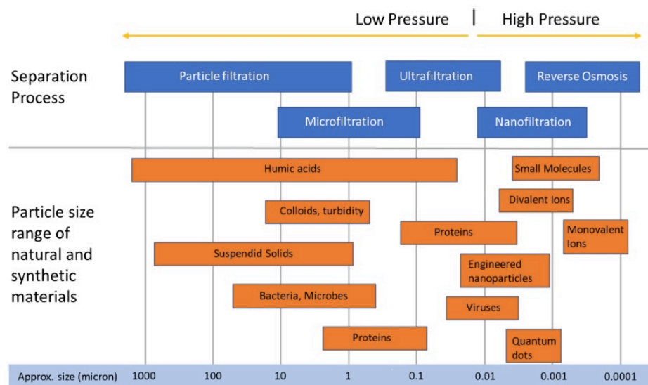
FIGURE 3. Comparison of water filtration membrane pore size with water contaminant size, reproduced from open source [12].
