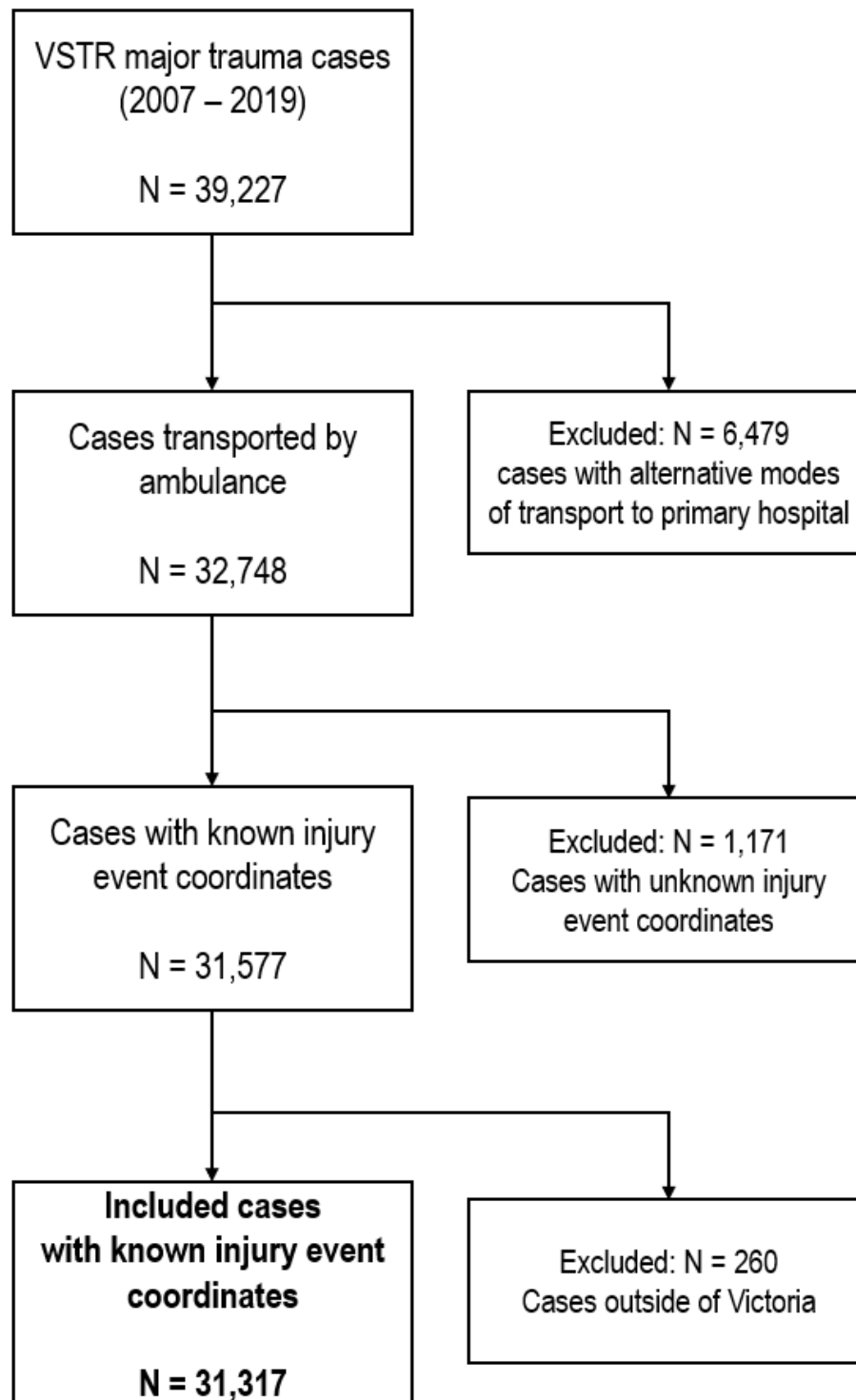
Figure 2: Data-filtering procedure.
