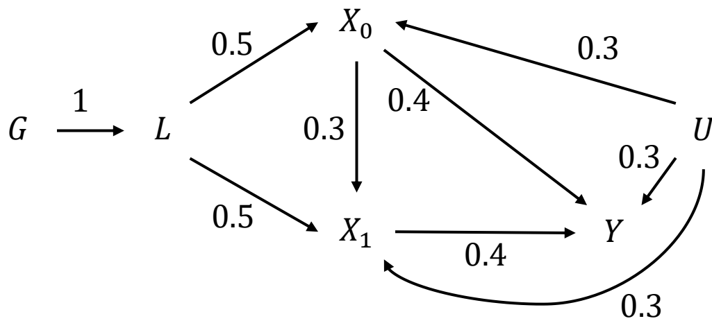
Figure 3: Simulated parameters. G , genotype; L , liability; X_0 , exposure measured at time 0; X_1 , exposure measured at time 1; Y , outcome; U , confounder.
