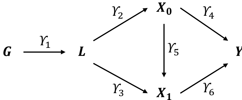
Figure 2: DAG showing the exposure liability in the context of two exposures and one outcome. G , genetic instrument; L , liability; X_0 , exposure measured at time 0; X_1 , exposure measured at time 1; Y , outcome; U , confounder.
