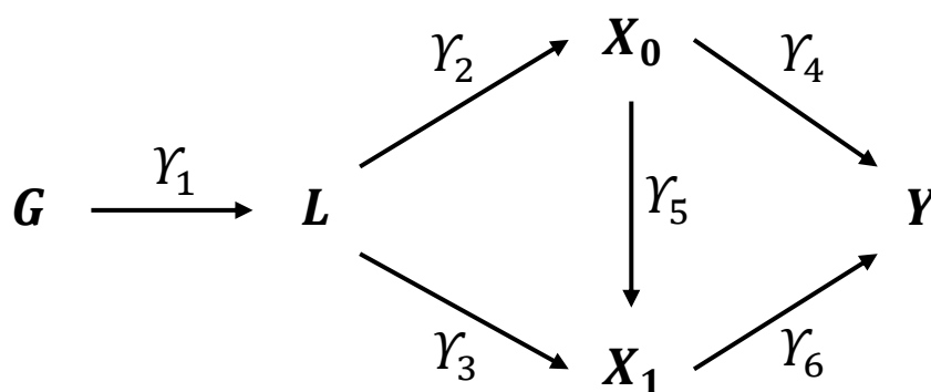
Figure A3: DAG showing the liability in the context of two exposures and one outcome. G , genetic instrument; L , liability; X_0 , exposure measured at time 0; X_1 , exposure measured at time 1; Y , outcome; U , confounder.
