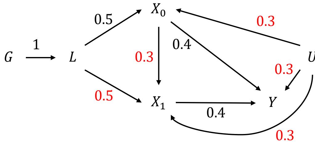
Figure A4: Simulated parameters. G , genotype; L , liability; X_0 , exposure measured at time 0; X_1 , exposure measured at time 1; Y , outcome; U , confounder. Parameters in red font are those that were varied.
