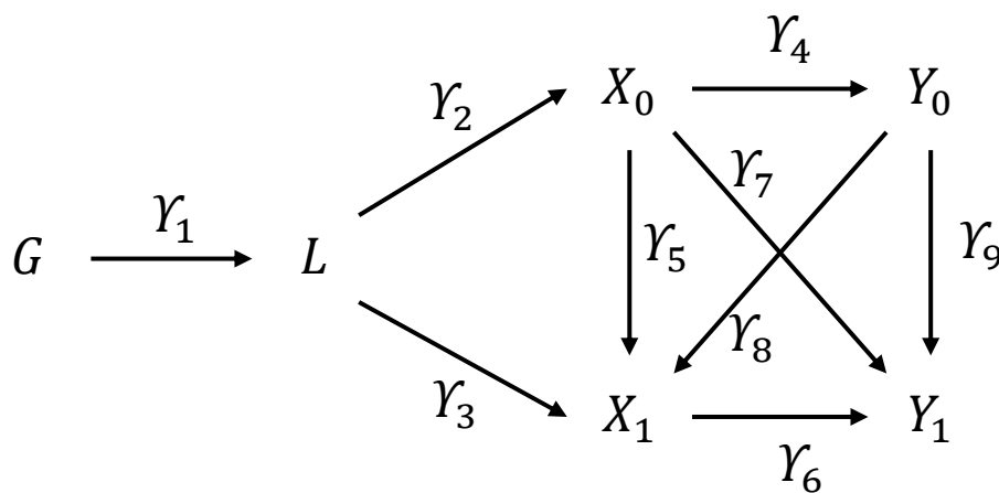
Figure A1: DAG showing the liability in the context of two exposures and two outcomes. G , genotype; L , liability; X , exposure; Y , outcome; U , confounder. Subscripts denote timepoint.
