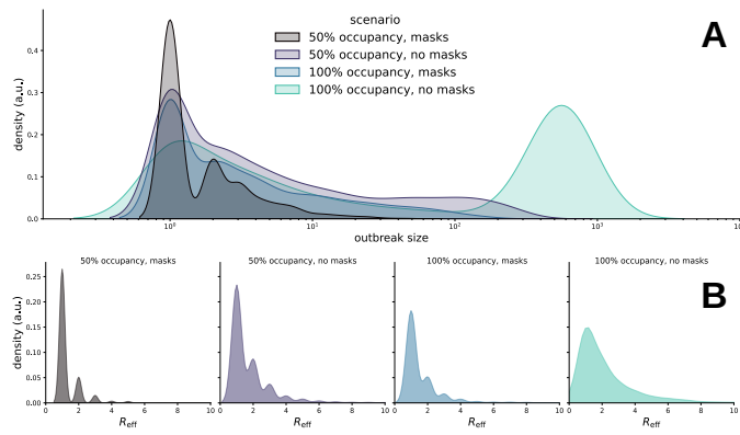
Fig. 2. Distribution of outbreak size (A) and effective reproduction number R_{eff} (B) over 10 000 simulations for different lecture hall occupancy levels and masking mandates at 80% vaccination coverage for students and faculty.
