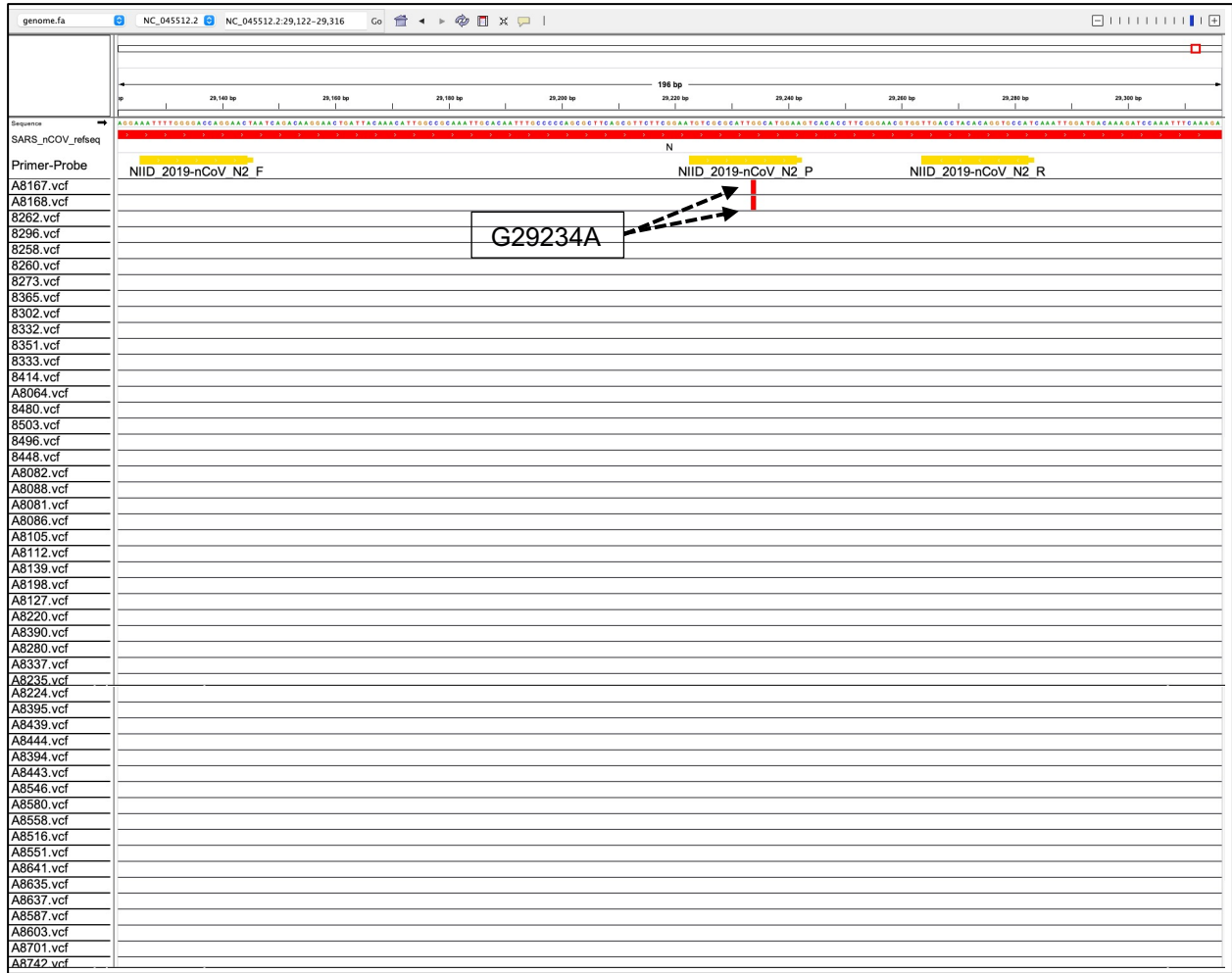
Supplementary Figure 1: Visualization of Variant Call Format (VCF) files of 63 samples (2 mutated samples and 61 other samples) collected from Kumamoto city area from September 1, 2021, to September 8, 2021, using Integrative Genomic Viewer (IGV). The red bar corresponding to the sample name depicts the presence of a mutation in that particular sample and the particular position corresponding to the reference sequence (NC_045512.2). The orange bar labelled "NIID_2019-nCoV_N2_P" reaches the region covered by the N2 probe suggested by Shirato et al. [14].
