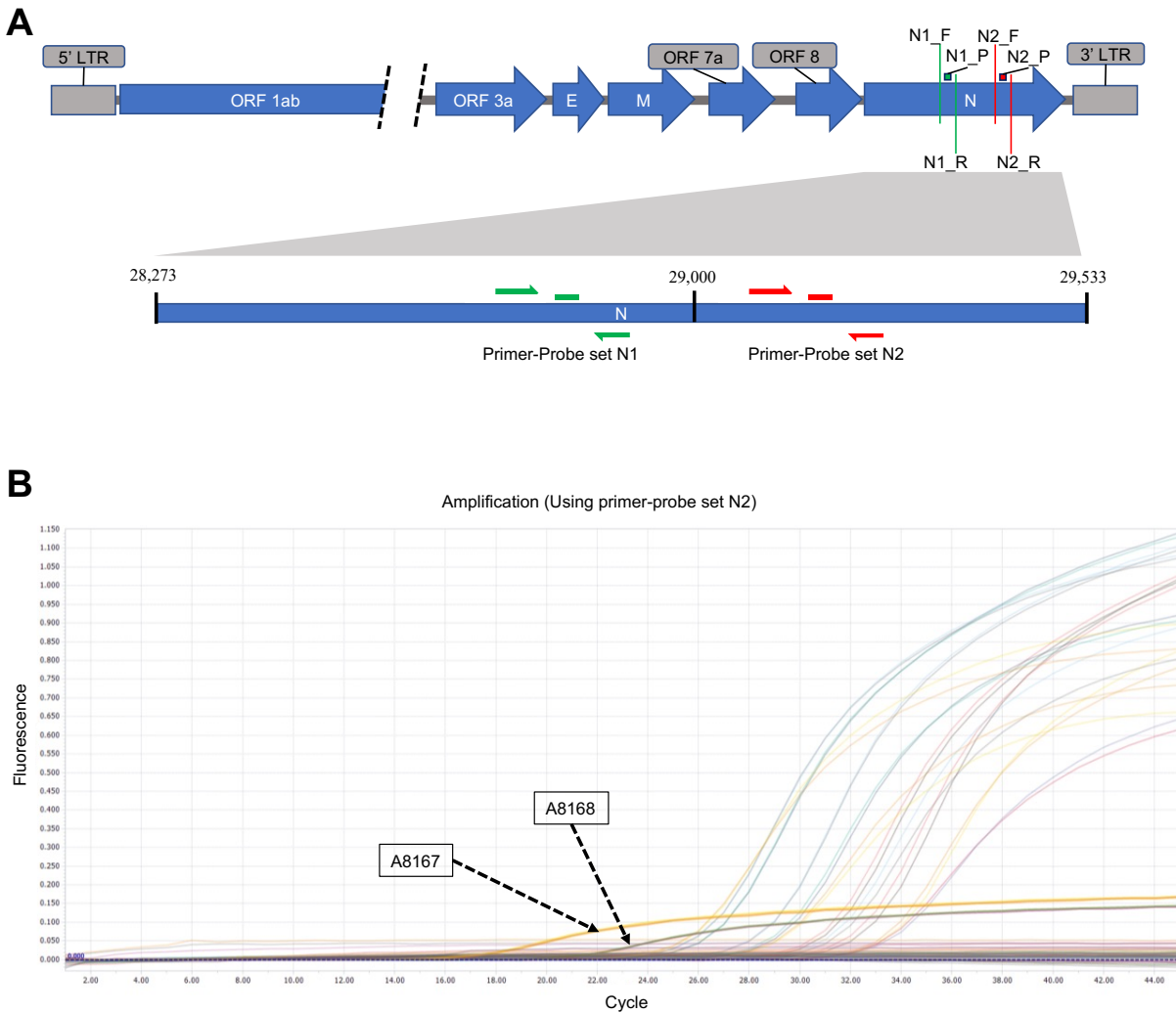
Figure 1: (A) Location of SARS-CoV-2 genome where the qRT-PCR primer-probe sets target for detecting SARS-CoV-2 in patient samples. Both primer-probe sets (N1 and N2) target the N protein-coding sequences. N1_F, N1_R, N1_P are the primers and probe of the N1 set and N2_F, N2_R, N2_P are the primers and probe of the N2 set (Figure not drawn to scale). (B) qRT-PCR curve to detect SARS-CoV-2 using NIID recommended N2 primer-probe set produced aberrant curve in two samples (A8167 and A8168) compared to other positive samples in the same run.
