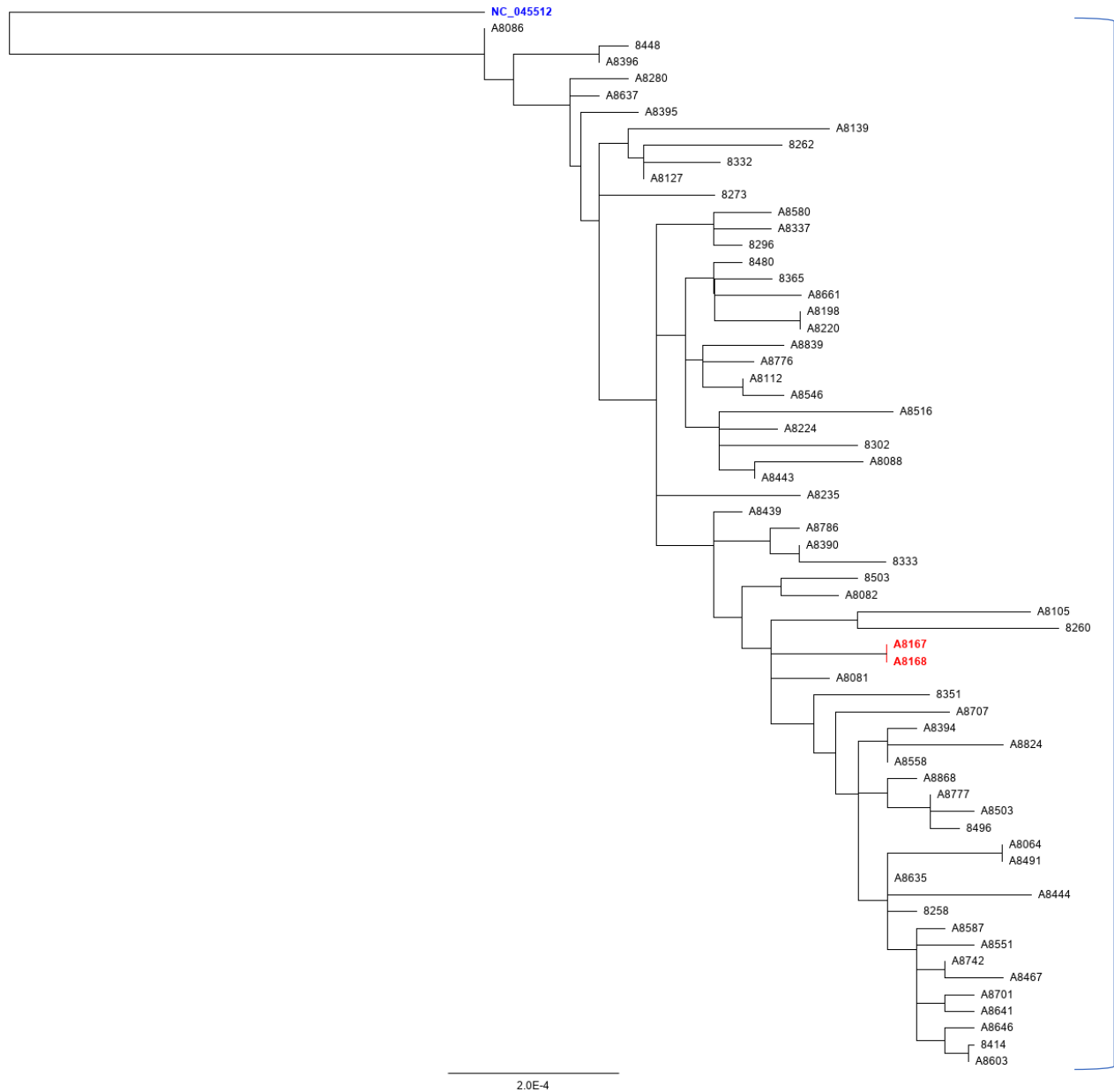
Figure 3: Maximum likelihood phylogenetic tree constructed using Geneious prime (version 2020.2.4) ( https://www.geneious.com/prime/ ) with 63 locally collected samples from Kumamoto city. The samples represent the same locality withing the same time frame. The scale bar indicates the number of substitutions per site. The Wuhan-hu-1 (NC_045512; heighted in blue) is placed as the root sequence of the tree and the red-highlighted samples contain the G→A mutation at 29234 loci of SARS-CoV-2 genome. AY is the alias used for B.1.617.2 lineage (Delta variant)
