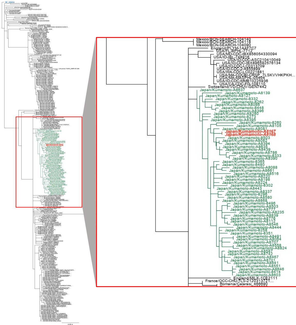
Figure 5: Maximum likelihood phylogenetic tree built in Geneious prime (version 2020.2.4) ( https://www.geneious.com/prime/ ) showed the relationships of viral strains collected from Kumamoto area from August 16, 2021 to September 8, 2021 with the viral strains having G29234A mutation from around the world. The Wuhan-hu-1 (NC_045512; heigted in blue) is placed as the root sequence of the tree and the green-highlighted samples represented the viral strains collected from the Kumamoto city. Red-bold faced viral strains (Zoomed in-Right panel) represent viral strains collected from Kumamoto area which contain G29234A mutation.
