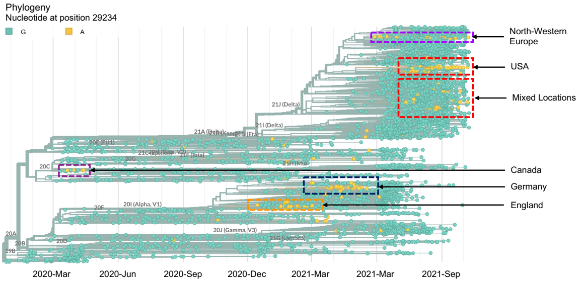
Figure 4: Nextstrain [37] generated phylogenetic tree with viral strains containing A allele at 29234 loci of the SARS-CoV-2 genome (highlighted in orange).
