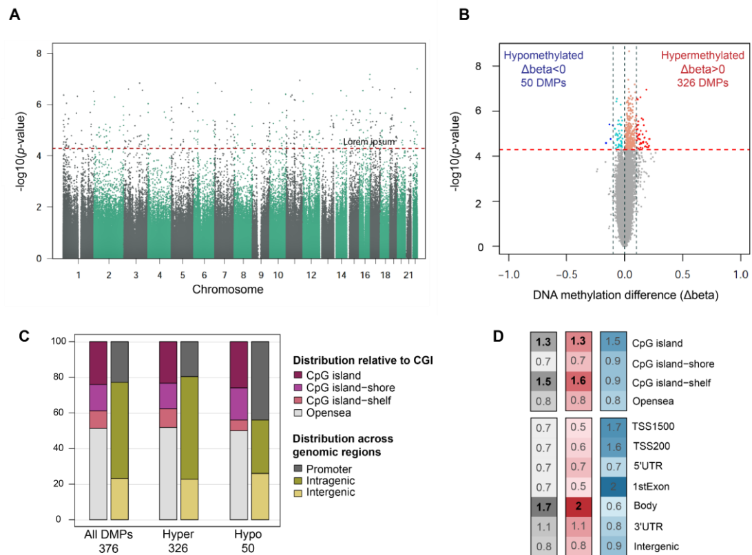
Figure 2. Distribution and annotation of differentially methylated positions (DMPs) between advanced neoplasia and no neoplasia pooled samples. A. Manhattan plot for differential methylation. The -\log_{10}(p\text{-value}) for the 741,310 probes analyzed are sorted by chromosome location. Significant DMPs (376) appear above the red dashed line (FDR 10%) B. Volcano plot showing the -\log_{10}(p\text{-value}) versus differences in methylation levels ( \Delta\beta : obtained by subtracting the DNA methylation levels (beta-values) of NN from AN). Significant hypermethylated ( \Delta\beta > 0 ) and hypomethylated ( \Delta\beta < 0 ) positions appear highlighted in color and above the red dashed line (FDR 10%). C. Distribution of the DMPs relative to CpG islands and functional genomic locations. D. Enrichment of DMPs in relation to CpG island annotation and functional genomic regions. The color scale indicates the fold enrichment of all DMPs (grey), hypermethylated (red), and hypomethylated (blue) positions. The bolded numbers indicate annotations that are enriched with respect to the distribution of probes on the MethylationEPIC array (one-sided Fisher's exact test p\text{-value} < 0.05 ). Functional characterization of probes according to the Methylation EPIC Manifest (R package version 0.6.0) (21): CpG island: region of at least 200bp with a CG content > 50\% and an observed-to-expected CpG ratio \geq 0.6 ; CpG island-shore: sequences 2 kb flanking the CpG island, CpG island-shelf: sequences 2 kb flanking shore regions, opensea: sequences located outside these regions, promoter regions (5'UTR, TSS200, TSS1500, and first exons), intragenic regions (gene body and 3'UTR), and intergenic regions. TSS200, TSS1500: 200 and 1500 bp upstream the transcription start site, respectively.
