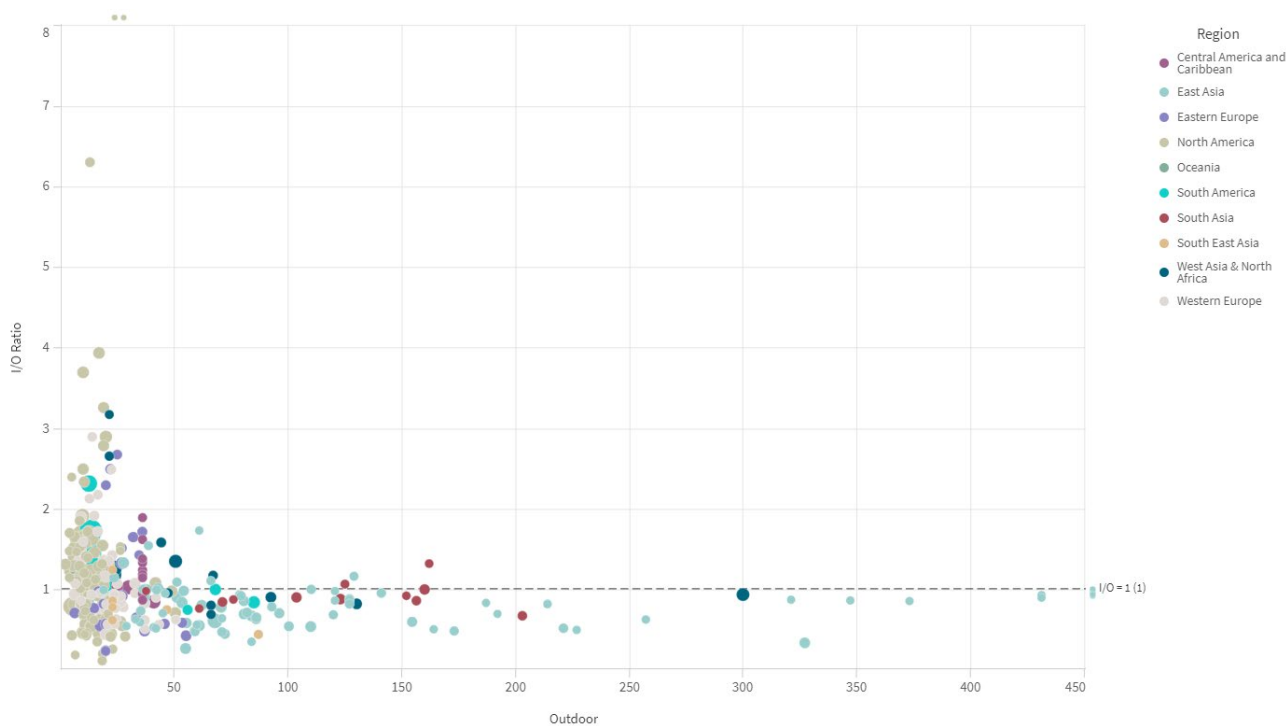
Figure 9. Indoor/outdoor ratios of PM_{2.5} with respect to outdoor (on site) concentrations ( \mu\text{g}/\text{m}^3 ). Four points outside the grid are shown that extend far beyond the axes ranges shown.
