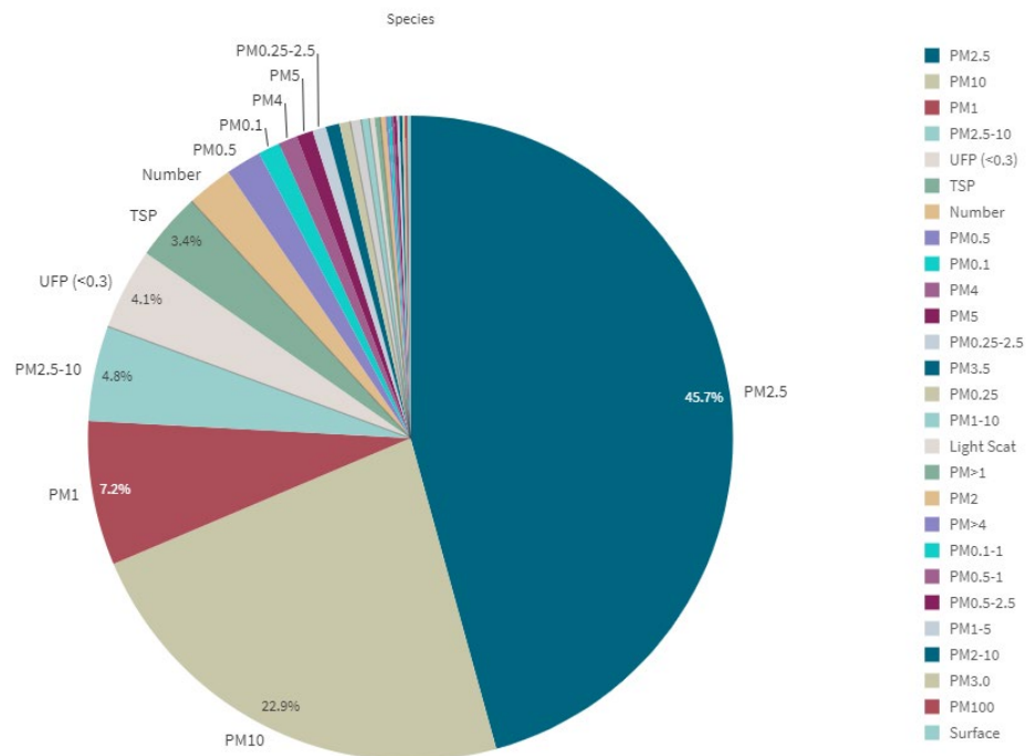
Figure 3. Fraction of studies investigating the different PM size fractions and other PM metrics.
