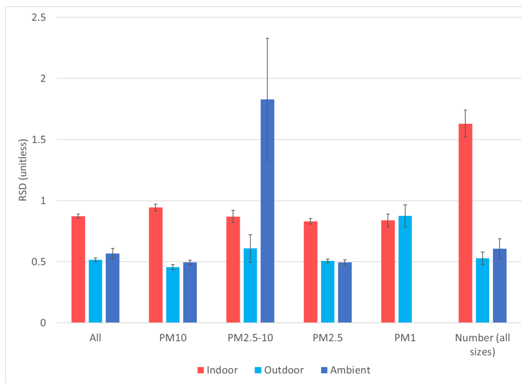
Figure 10. Variability of indoor, outdoor, and ambient monitor measurements expressed as relative standard deviation (SD/Mean). Error bars are standard errors. Only means and SD reported in the studies are included, without calculated ones.
