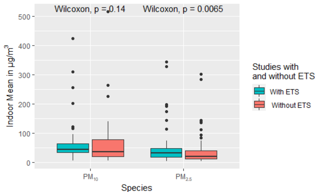
Figure 11. Box plot of indoor mean values for PM 10 and PM 2.5 for studies with and without ETS. Statistics labeled 'Without ETS' are restricted to measurements in homes without environmental tobacco smoke, while statistics labeled 'With ETS' contains measurements in homes with and without environmental tobacco smoke. Additional descriptive statistics for these PM species as well as other size fractions can be found in the in the supplementary Information (Table S3)
