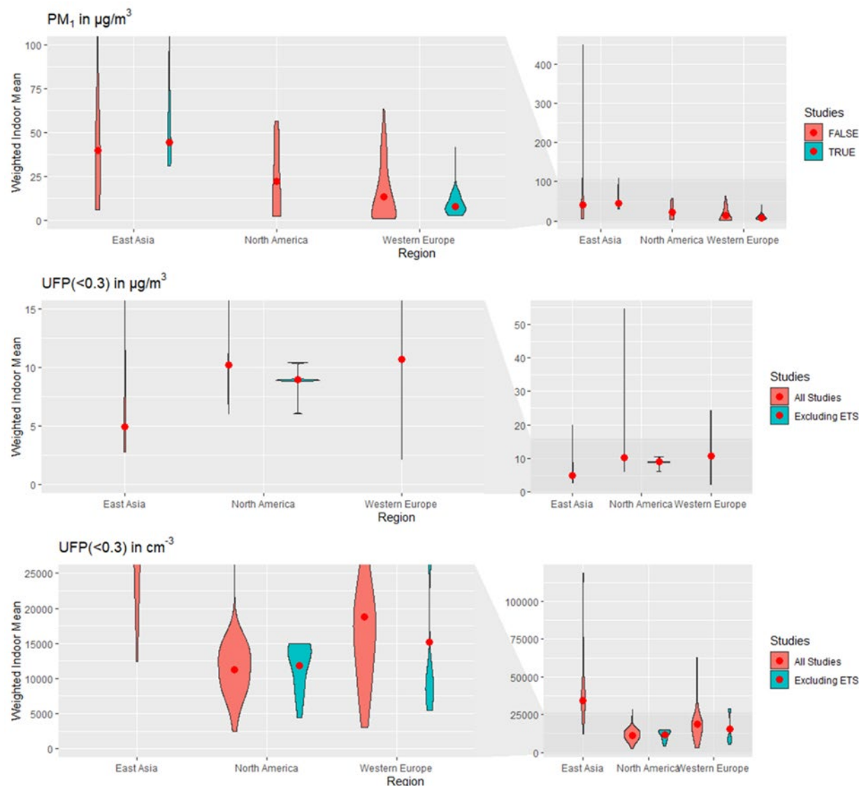
Figure 6. Weighted frequency distributions of means for PM 1 , UFP (in µg/m 3 and cm -3 ) for East Asia, North America and Western Europe. The red points are displaying the weighted indoor mean of means, within a size fraction. Studies labeled 'Excluded ETS' are restricted to mean measurements in homes without environmental tobacco smoke. Left panels show magnified region of right panels
