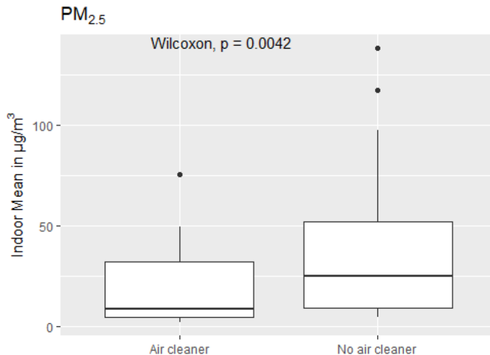
Figure 12. Box plot of indoor mean values for \text{PM}_{2.5} for studies reporting results both with and without air cleaners. Statistics labeled 'No air cleaner' are restricted to measurements in homes without air cleaners, yet the corresponding study contains measurements with air cleaners. Statistics labeled 'Air cleaner' contains measurements in homes with air cleaners. Additional descriptive statistics for this PM species as well as other size fractions can be found in the in the supplementary Information (Table S4)
