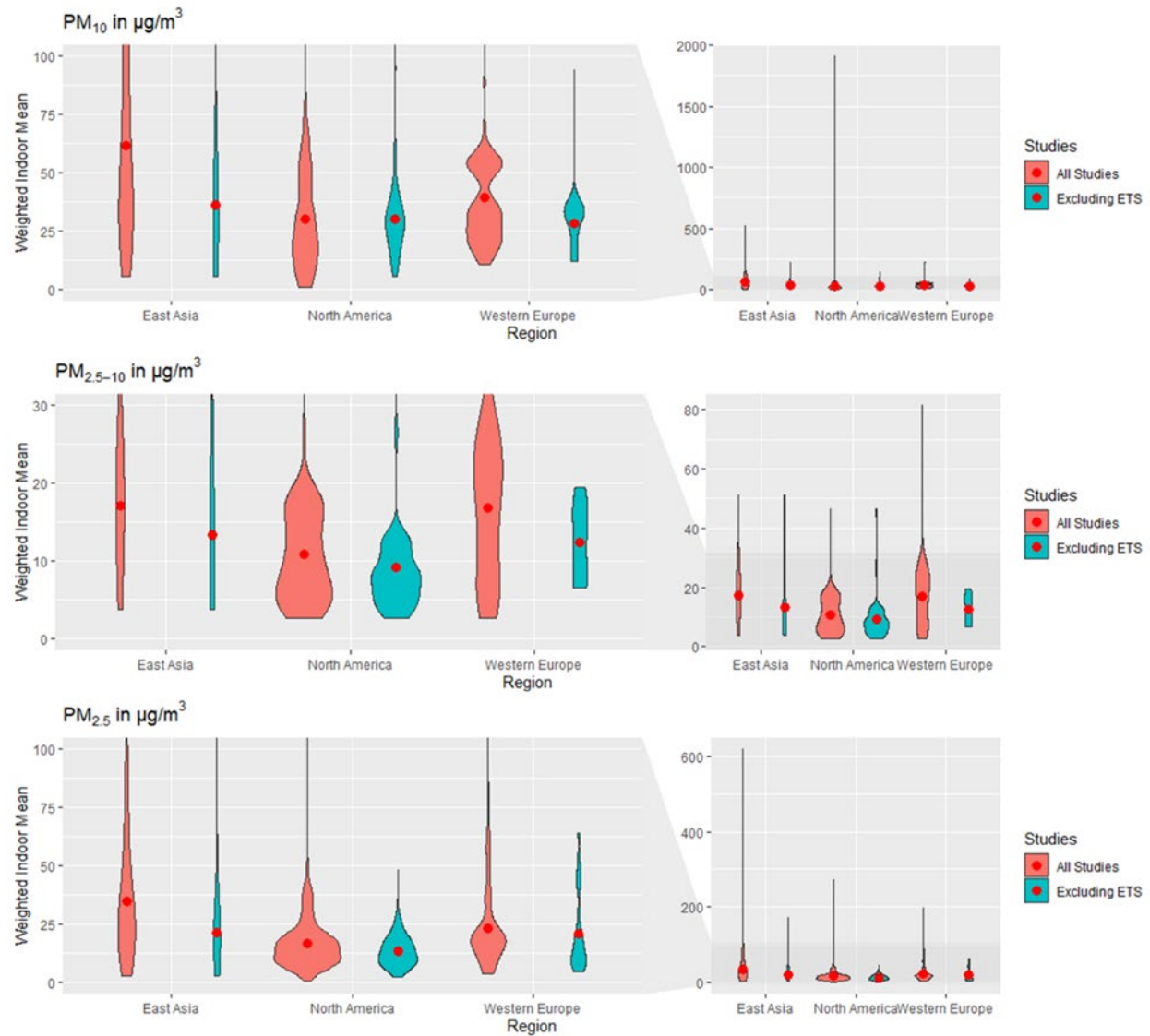
Figure 5. Weighted frequency distributions of means for PM_{10} , PM_{2.5-10} and PM_{2.5} for East Asia, North America and Western Europe. Width is proportional to the number of means, within a size fraction. The red points are displaying the weighted indoor mean of means. Studies labeled 'Excluded ETS' are restricted to mean measurements in homes without environmental tobacco smoke. Left panels show magnified region of right panels.
