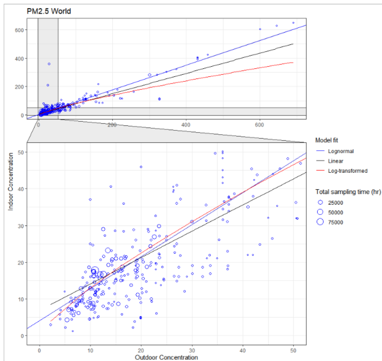
Figure 8. Scatterplot of mean indoor and outdoor (on site) concentrations pairs for \text{PM}_{2.5} (in \mu\text{g}/\text{m}^3 ). Circle size indicates the total sampling time of the measurements (in hours) across all sampled buildings for a pair of mean concentrations in a study, which were used as weights in the regressions. The Model Fit lines show 3 different fitting approaches: lognormal regression, simple linear regression on unmodified data, and linear regression on log-transformed data. Bottom graph shows magnified region of top graph.
