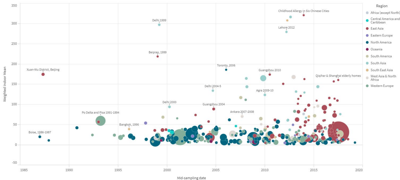
Figure 7. Weighted study means of PM 2.5 ( \mu\text{g}/\text{m}^3 ) by mid-point of sampling campaign and region. Marker size is proportional to total study sampling time.
