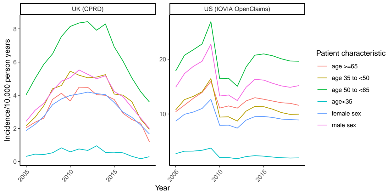
Figure 2: Incidence of ASAD per 10,000 person years in UK (CPRD) and US (IQVIA OpenClaims), stratified by patient characteristics. Note that the y-axis scales differ.
