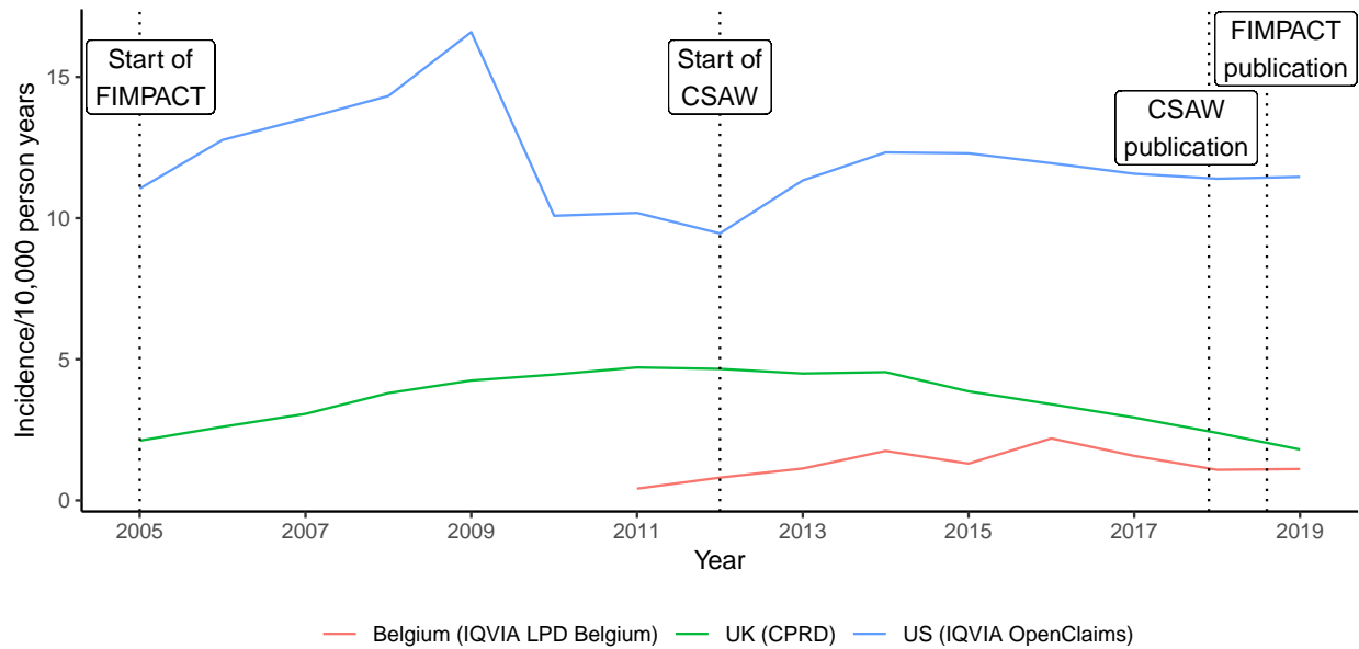
Figure 1: Incidence of ASAD per 10,000 person years in Belgium, UK and US. The FIMPACT[2] trial recruited in Finland from 2005 to 2013 and published in July 2018. The CSAW[1] trial recruited in the UK from 2012 to 2015 and was published in January 2018. Both trials did not find evidence of a clinically important difference compared to diagnostic arthroscopy (i.e. placebo surgery).
