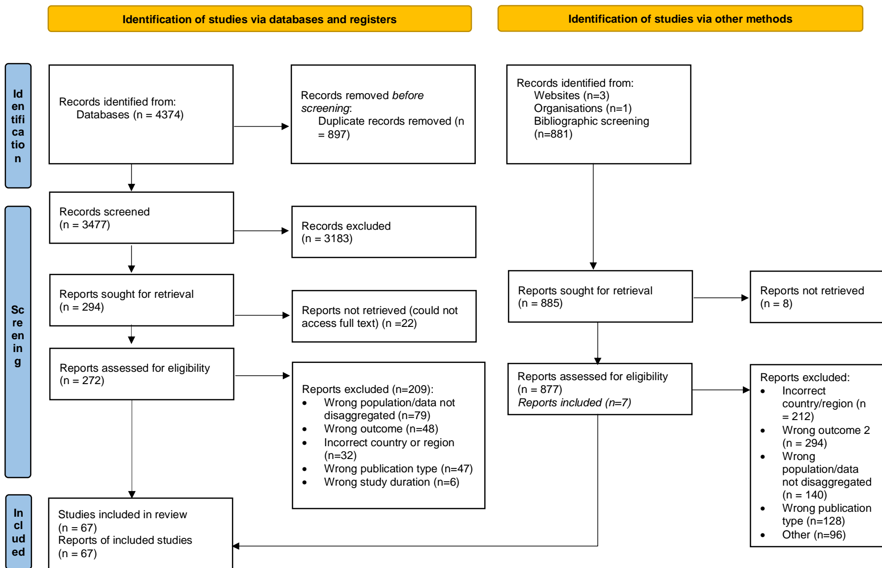
Figure 1. Study selection process, as shown by PRISMA 2020 flow diagram for new systematic reviews which included searches of databases, registers, and other sources. Reproduced from: (18)
