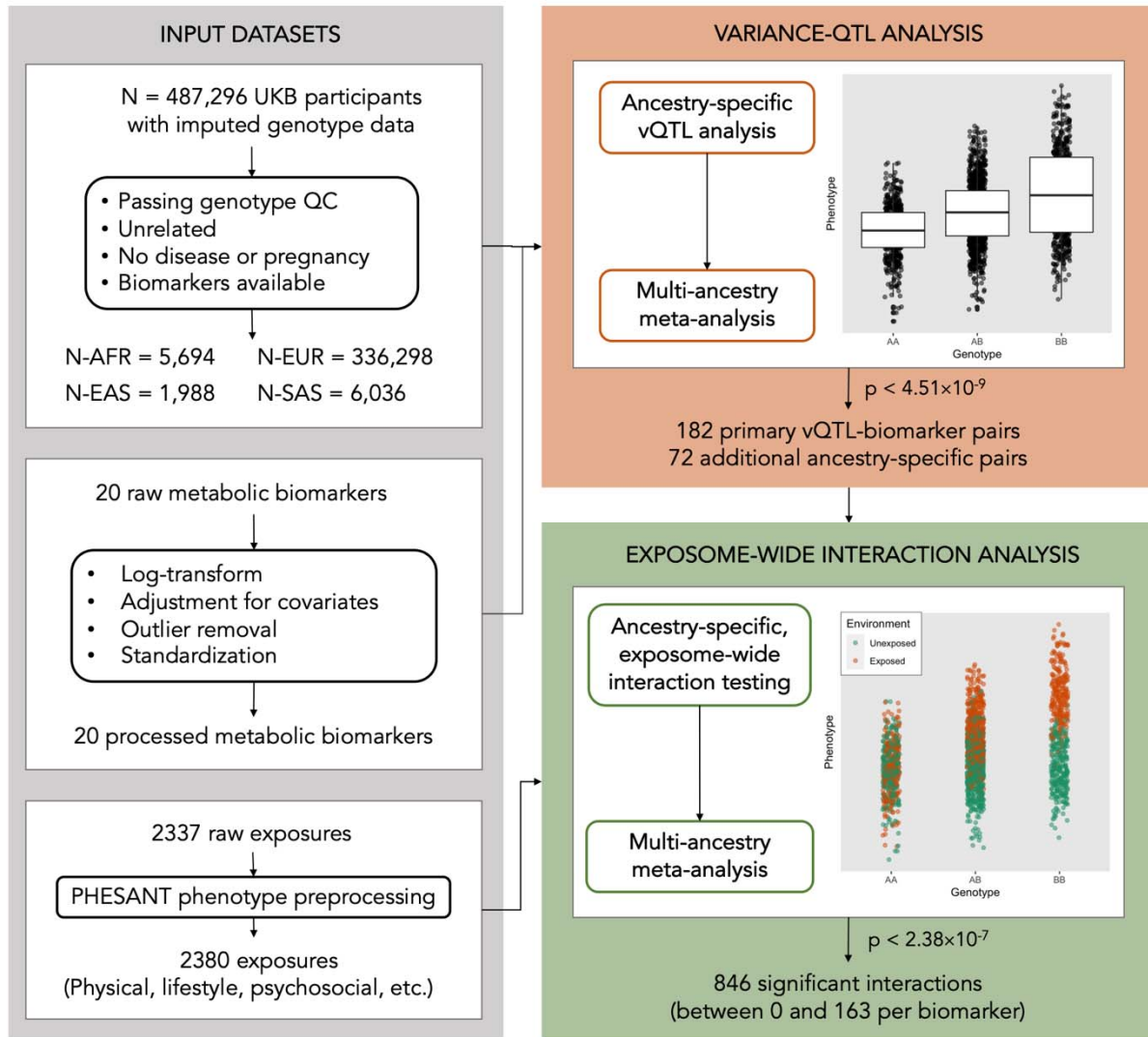
Figure 1: Analysis workflow.
