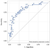
Answer: \frac{1}{2}
