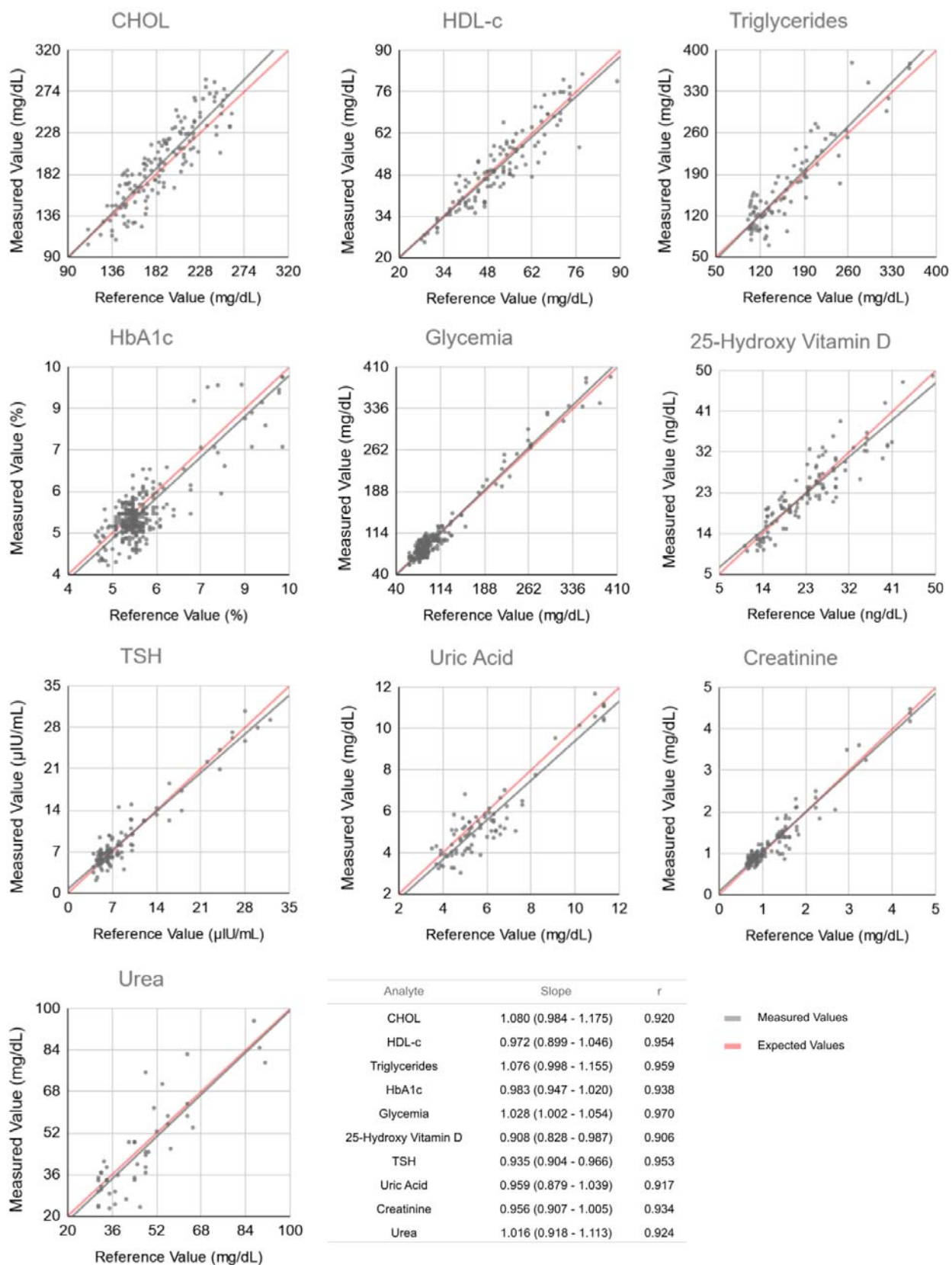
Figure 1 - Regression Parameters and Correlation between reference and proposed method. Correlation between methods was extremely high ( r > 0.9 ) for all analytes.
