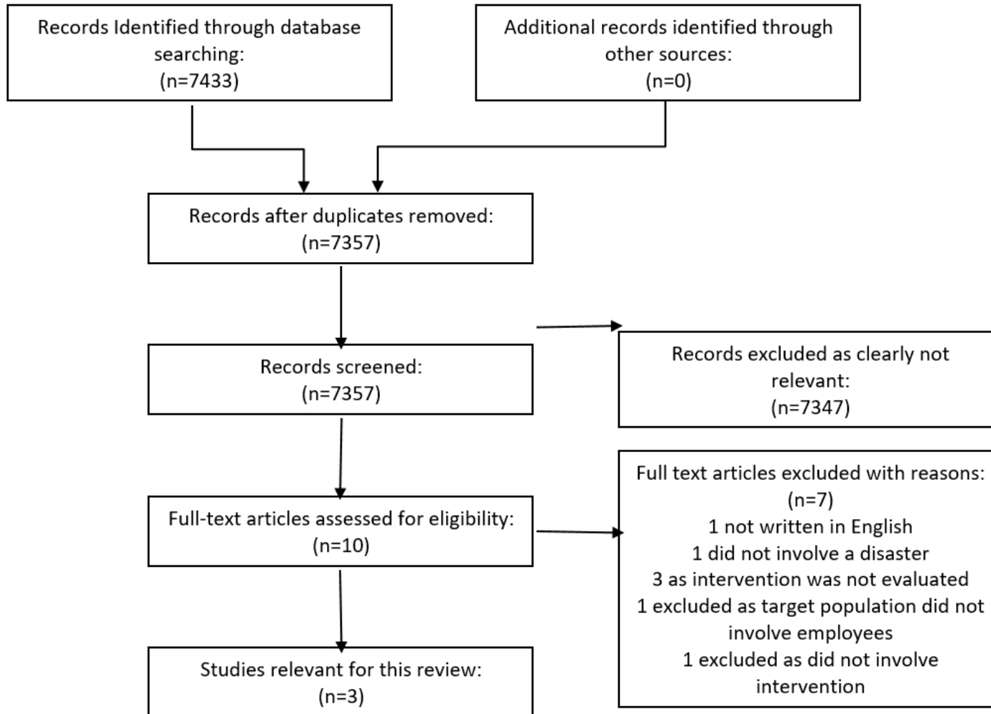
Fig. 1 Prisma Flow Diagram of Literature Search
