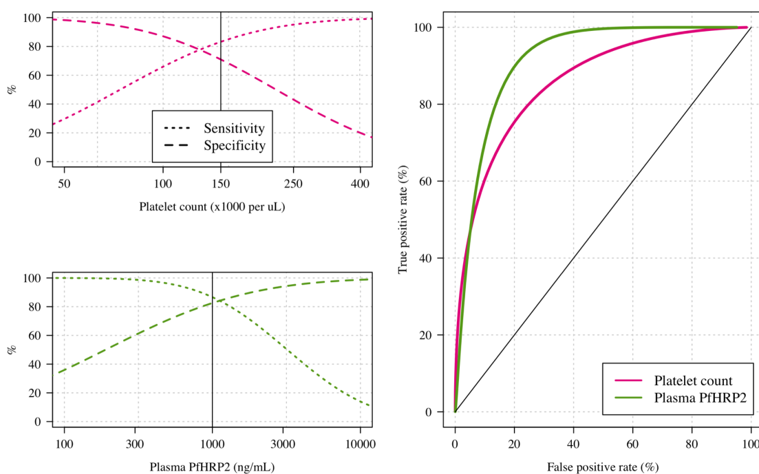
Figure 1: The diagnostic value of platelet counts (pink) and plasma PfHRP2 concentrations (green) estimated using data from 2,063 patients diagnosed with severe falciparum malaria in three studies. Sensitivities (dotted lines) and specificities (dashed lines) are estimated under a Bayesian parametric two-component latent class model which assumes the same sensitivity and specificity for each biomarker across the three studies (African children: Kilifi, Kenya and Kamapala, Uganda; Asian adults: Bangladesh). For the platelet count, thresholds correspond to upper limits, whereas for the PfHRP2 concentration the thresholds correspond to lower limits.
