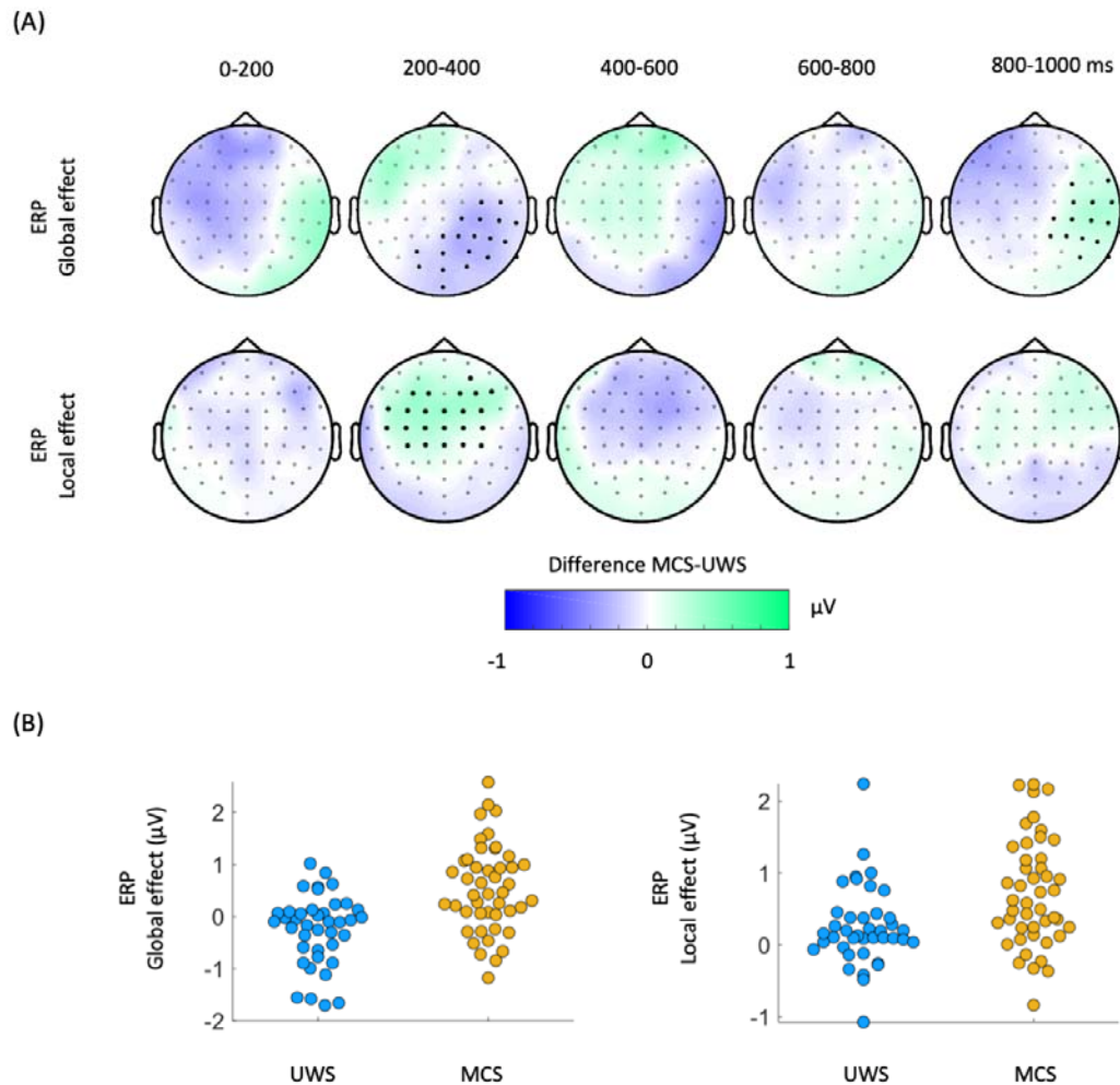
Figure 2. Auditory event-related potentials (ERPs) in the global and local effect. (A) Scalp topographies indicate the average group differences between MCS and UWS patients. Thick electrodes indicate a clustered effect (Monte Carlo p < 0.05 ). (B) Average of the clustered effects per patient, in the ERP global effect (main positive cluster: p = 0.0001 , Z = 3.684 , latency = 800-850 ms; main negative cluster: p = 0.0013 , Z = -3.1905 , latency = 280-336 ms) and ERP local effect (main positive cluster: p = 0.0011 , Z = 3.4416 , latency = 236-328 ms). ERPs: auditory event-related potentials, MCS: minimally conscious state, UWS: unresponsive wakefulness syndrome
