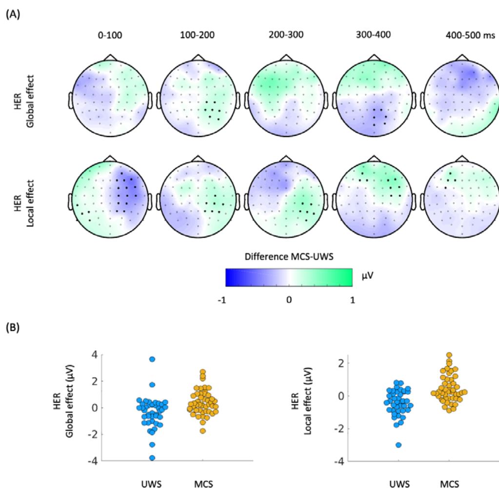
Figure 3. Heartbeat-evoked responses (HERs) in the global and local effect. (A) Scalp topographies indicate the average group differences between MCS and UWS patients. Thick electrodes indicate a clustered effect (Monte Carlo p < 0.05 ). (B) Average of the clustered effects per patient, in the HER global effect (main positive cluster: p = 0.0037 , Z = 3.0173 , latency = 112-130 ms; main negative cluster: p = 0.0058 , Z = -3.0173 , latency = 340-360
