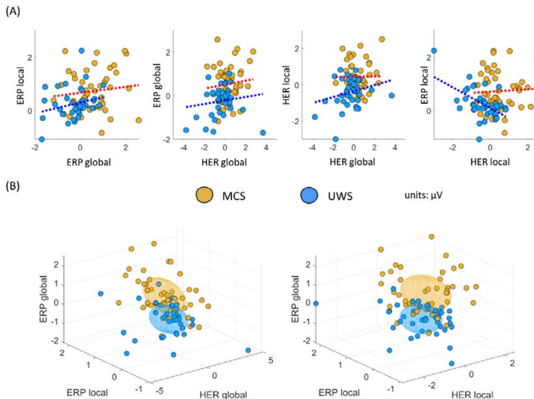
Figure 4. Multi-dimensional analysis of the clustered effects found when comparing MCS and UWS patients. (A) Pairwise comparison between all possible combinations for ERPs and HERs, for local and global effects. Individual points corresponding to a single patient, and dotted line indicates the trend, separately per diagnosis. (B) Three-dimensional representation of the clustered effects: left panel for ERP global, ERP local and HER global; and right panel for ERP global, ERP local and HER local. Each ellipsoid was constructed per diagnostic group, centered in the group means with ratio defined by the standard deviations, for the respective dimensions. HERs: heartbeat-evoked responses, ERPs: auditory event-related potentials, MCS: minimally conscious state, UWS: unresponsive wakefulness syndrome
