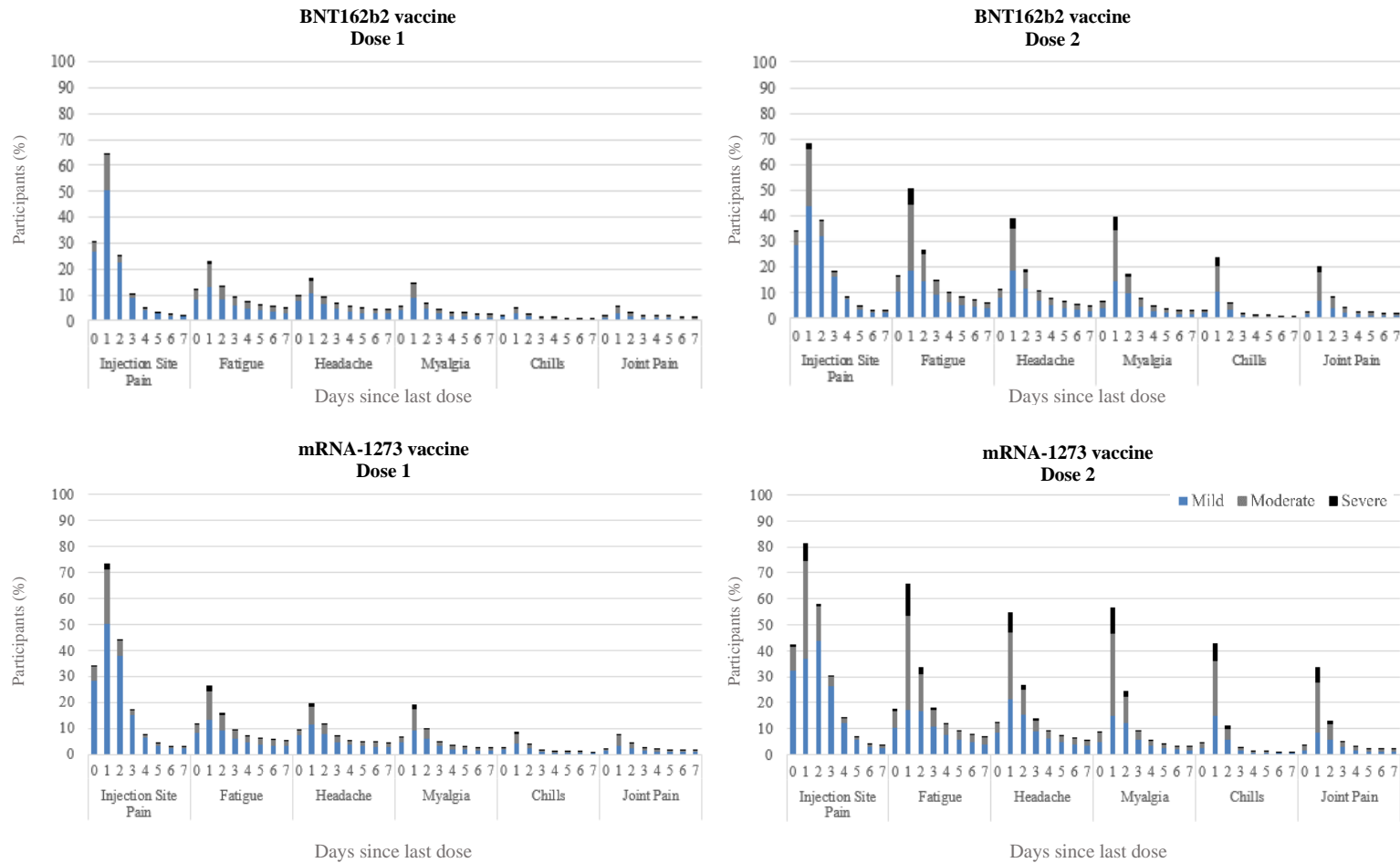
Figure 1: Local and systemic reactions* to mRNA COVID-19 vaccine reported in v-safe, by manufacturer, dose, days after vaccination, and severity†
