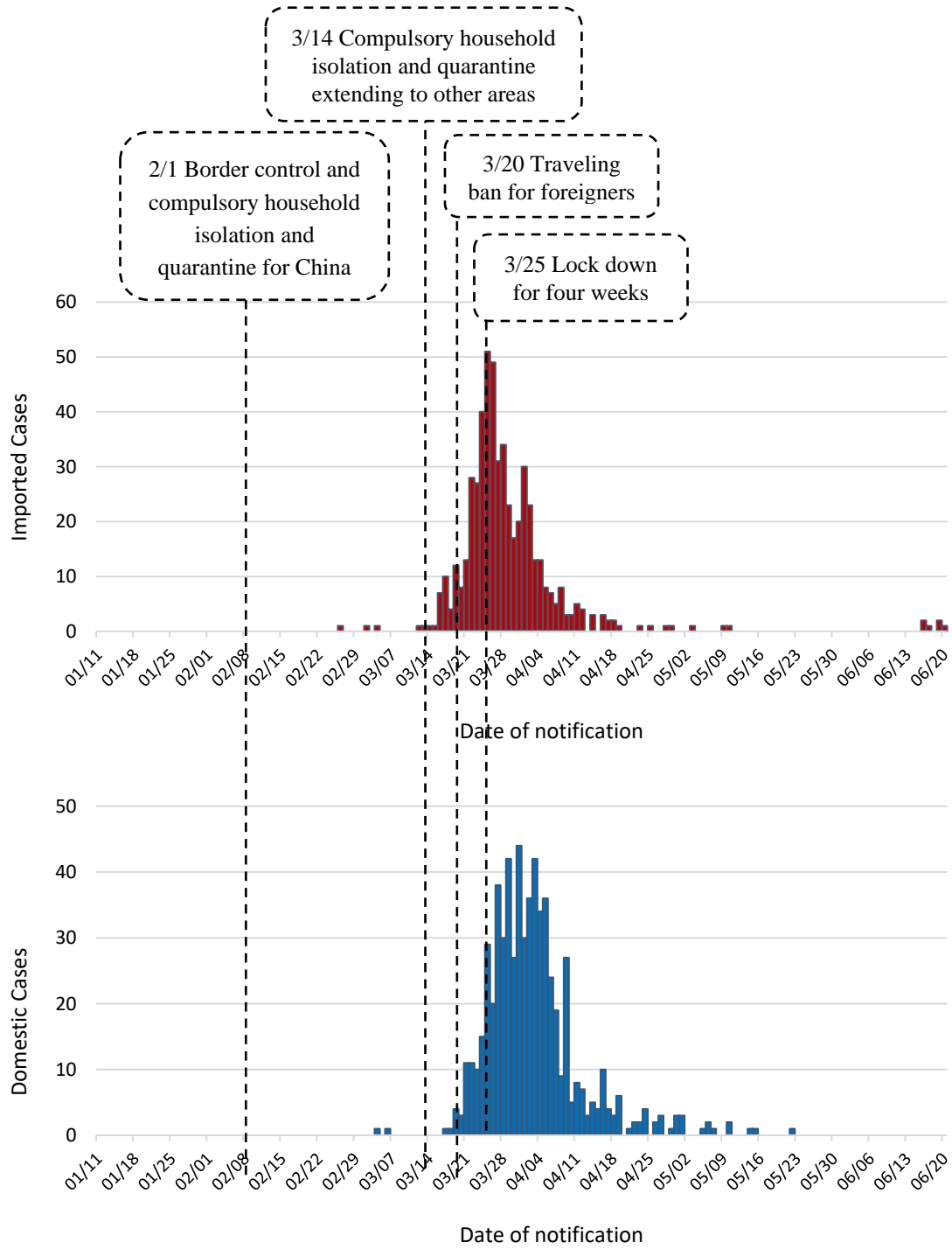
Supplementary fig 6. Epidemic curve of covid-19 outbreak in New Zealand by types of cases
