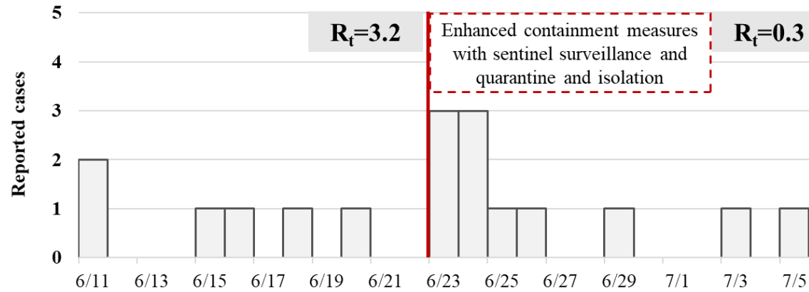
(a) Empirical epidemic curve of the outbreak
