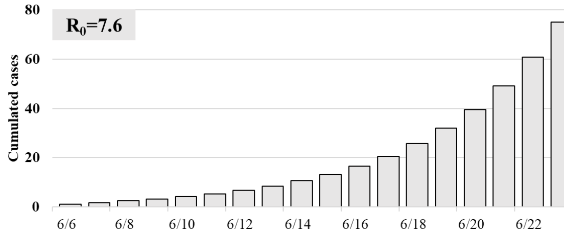
(b) Epidemic curve reconstructed from the transmission dynamic of covid-19
