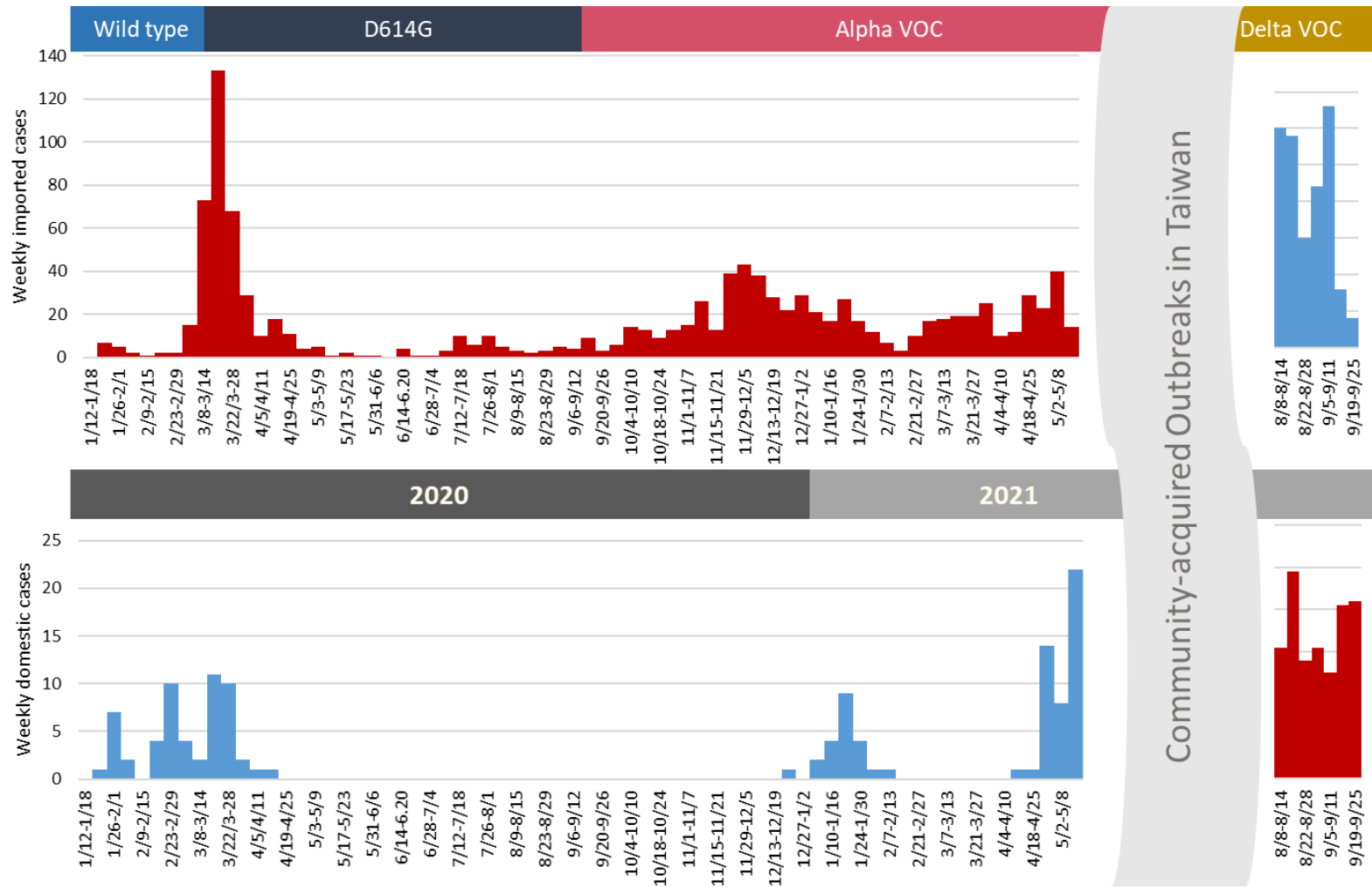
Fig 1. Covid-19 epidemics in Taiwan for periods without CAO by origin of cases (imported vs domestic)
