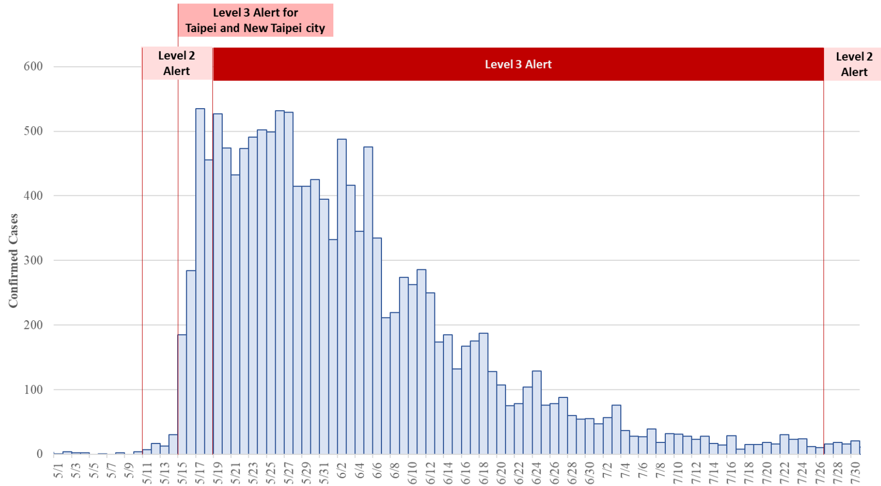
(a) Epidemic curve
