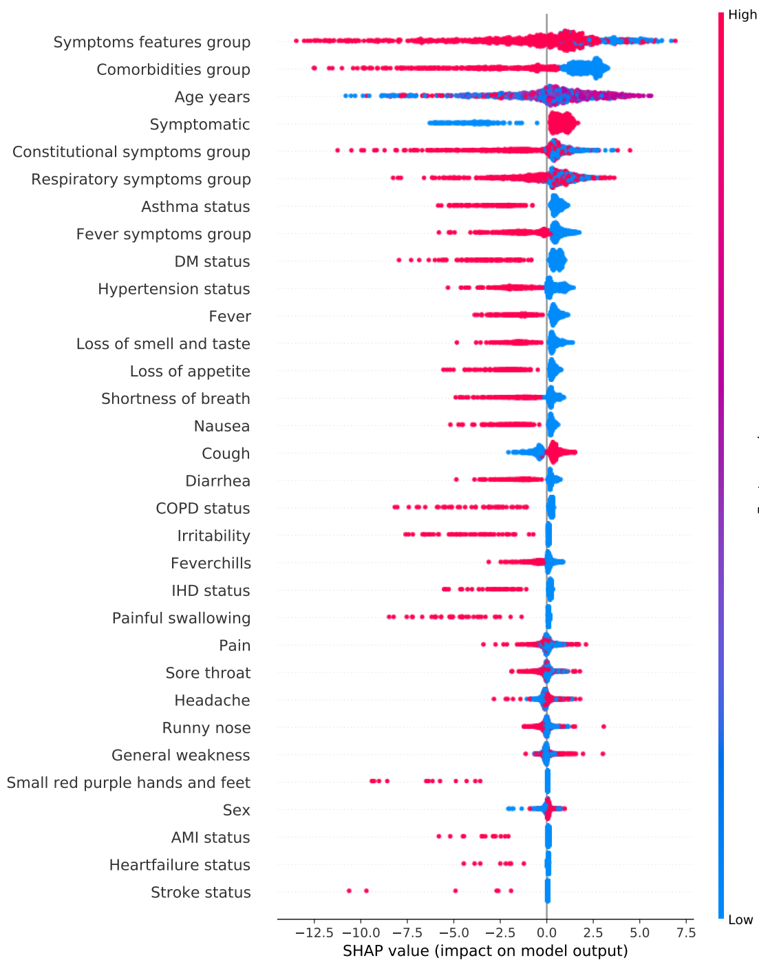
Figure 10: Scaled SHAP feature importance for OCSVM at-risk prediction
