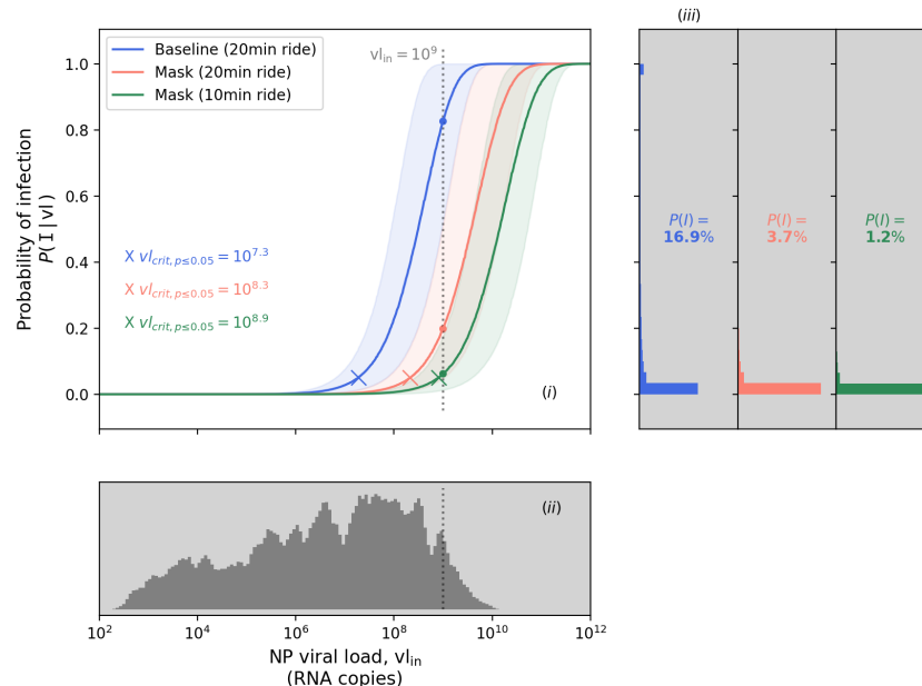
Figure 3: Probability of infection in the ski cabin scenario, and related dependency on the viral load. Results assume the index host was infected with the Delta VOC and none of the occupants were vaccinated. (i) Expected probability of infection for a given viral load value, with mean (solid line) and 90% CI (shaded area). Comparison between the baseline scenario (blue curve) and situations with stricter set of measures. The x markers denote the critical viral load v_{crit, p \le 0.05} in each situation. The dotted line correspond to the hypothetical viral load of the infected (index) host. (ii) Histogram of the viral load data from [23]. The vertical axis corresponds to the probability density function of the adopted distribution. The dotted line indicate the the hypothetical viral load of the infected (index) host. (iii) Set of histograms of the conditional probability of infection P(I|v) , one for each scenario, showing the results of the MCS, including the integration on the full range of viral load data in [23]. The P(I) values shown in the middle of each histogram plot indicate the full probability (as per Eq. 19).
