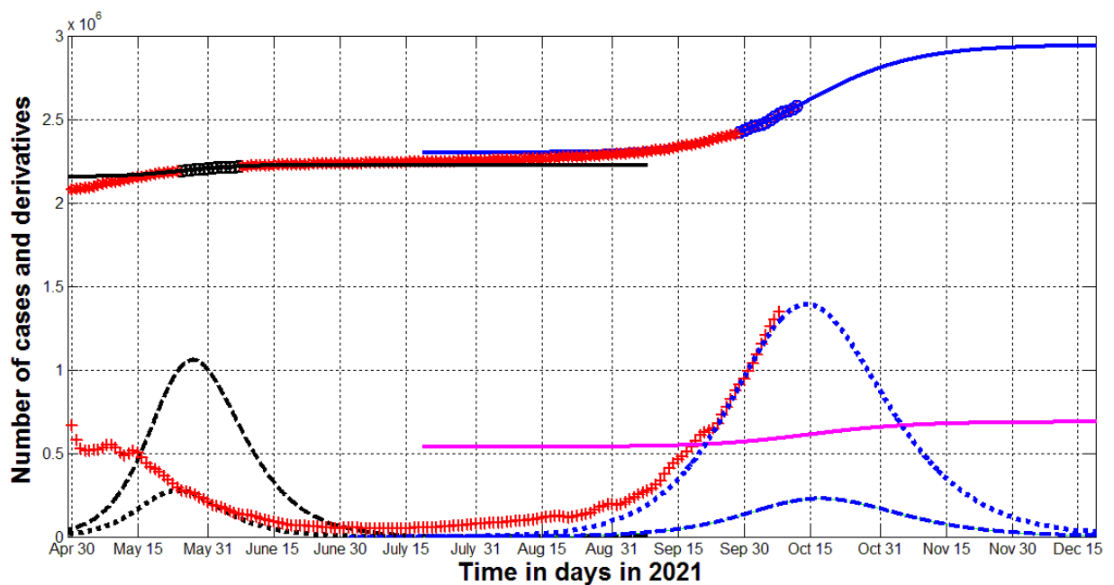
Figure. 11-th and 12-th waves of the COVID-19 pandemic in Ukraine in the summer and autumn of 2021.
