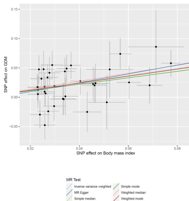
Figure 2. Effects of BMI on GDM from MR analyses. Each point corresponds to an independent SNV (genetic instrument), plotted according to the effect on BMI (on the x-axis) and the effect on GDM (log-OR, on the y-axis). Horizontal and vertical bars represent the standard errors of effect estimates. The coloured regression lines represent the effect of BMI on GDM from six MR models.
