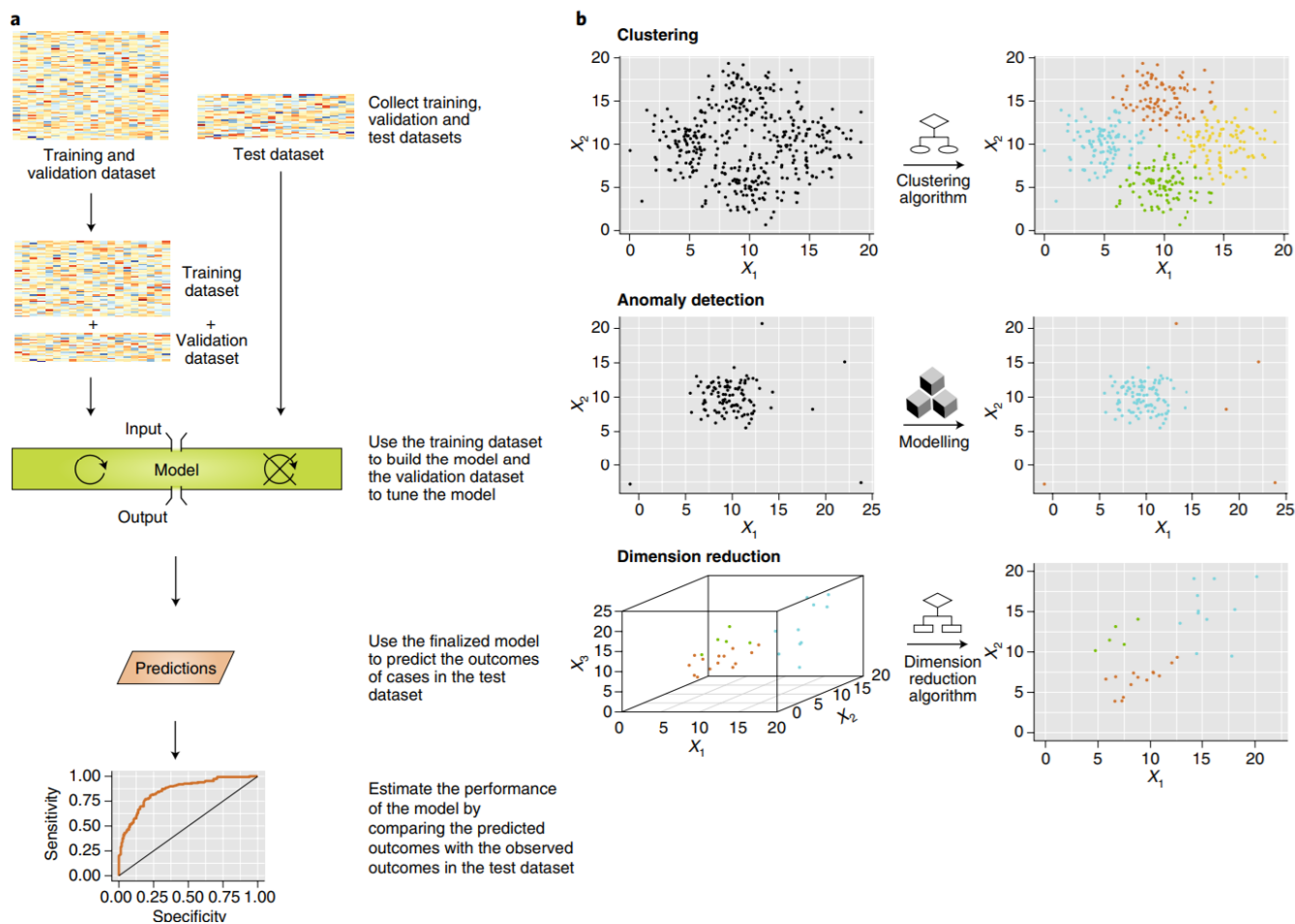
Figure 1: | Supervised and unsupervised machine learning. a , General workflow of supervised machine-learning approaches. First, training and test datasets are collected. Next, part of the training set is used to build the prediction model, and the other part to tune and validate the model (circular arrow). After the machine-learning model is finalized (crossed-out circular arrow), the established model is used to generate predictions on the test dataset and the model’s performance is estimated by comparing the predicted outcomes with the observed outcomes for the test dataset. b , Unsupervised machine learning includes clustering, anomaly detection and dimensionality reduction. Clustering algorithms group data points with similar measurements into clusters. Anomaly detection identifies outliers in the dataset. Dimensionality reduction reduces the number of random variables used to describe the data; for example, by representing an image with thousands of parameters as a smaller vector of summary features. The resulting summary vector preserves the important information in the raw data; for example, summary vectors from similar images will bear more resemblance than those obtained from irrelevant images
