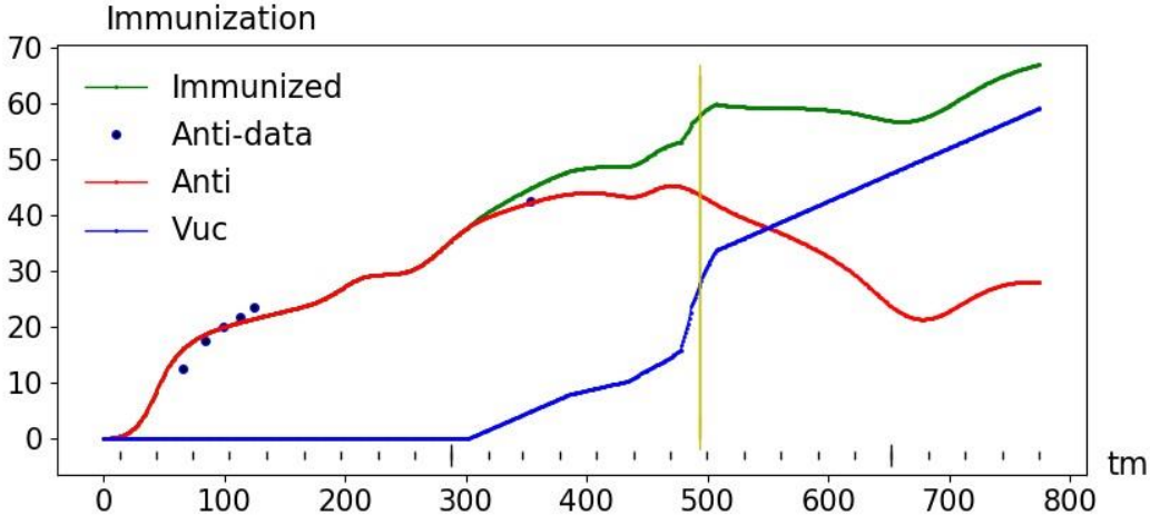
Fig. 13. The forecast of immunization of the Moscow population in the fourth wave from 25.07.2021. Vuc(t) – preset control, the percentage of vaccinated (corresponds to the rate of vaccination 12 thousand/day). Anti(t) – forecast of the percentage of those recovered who retained their immunity by the time t . Immunized(t) – forecast of the percentage of the resistant (vaccinated and recovered with immunity)
