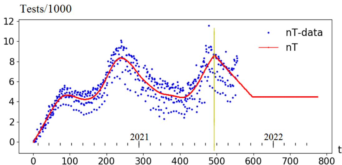
Fig. 15. Number of tests per thousand: data fitting and preset scenario for the fourth wave forecast from 25.07.2021 (to the right of the yellow line).
