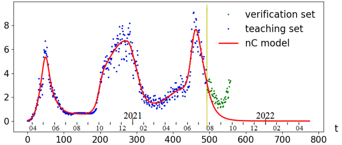
Fig. 8. Third wave forecast for Moscow from 25.07.2021.
