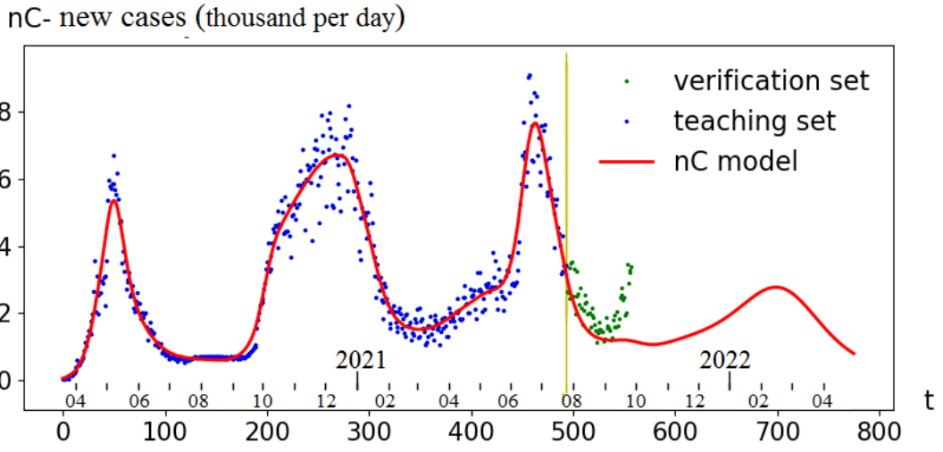
Fig. 12. Fourth wave forecast for Moscow from 25.07.2021, and its comparison to real (the green dots) data, up until 27.09.2021
