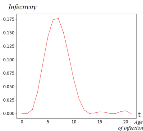
Fig. 1. Normalized (integral equals one) infectivity as a function age of infection (days).
