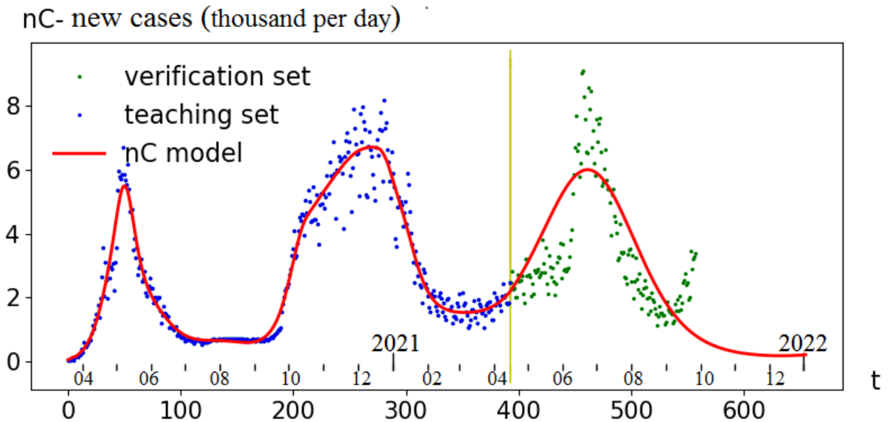
Fig. 5. Forecast of the third wave of new cases of infection in Moscow from 15.04.2021. Blue dots – training set, red curve – model, green dots – (verification?) testing set (up until 20.09.2021).
