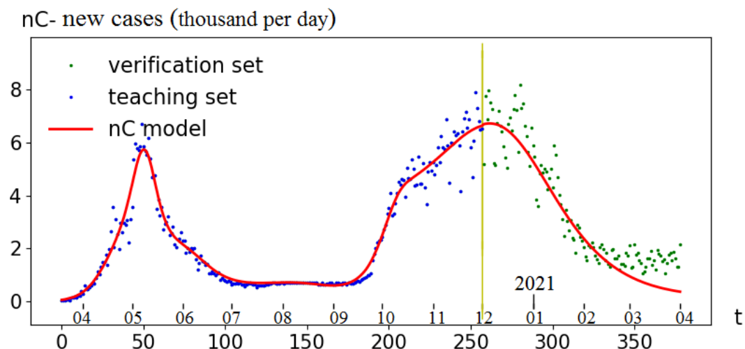
Fig. 4. Forecast of new cases of infection in Moscow from 01.12.2020. Blue dots – training set, red curve – the model, green dots – testing set.
