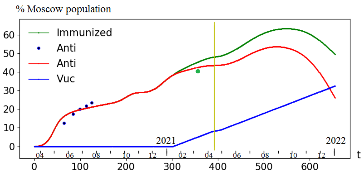
Fig. 6. Immunization of the population of Moscow. Vuc(t) – preset management, the percentage of vaccinated (corresponds to the rate of vaccination of 12 thousand/day). Anti(t) – forecast of the percentage of those recovered who retained their immunity by the time t . Immunized(t) – forecast of the percentage of "immunized" (vaccinated and recovered with immunity). Blue dots (percentage of carriers of antibodies, i.e., those who had recovered) were used for identification, the green dot was left for verification.
