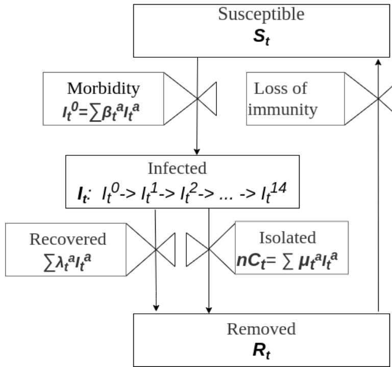
Fig. A2. Model SI_{15}RS . The removed (immune) become susceptible again due to loss of immunity.
