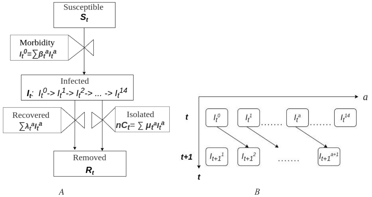
Fig. A1. A. Model SI_{15}R : I (infected) are divided into 15 subgroups. B. An illustration of the dynamics of the groups of infected, determined by a shift in the age of infection ( a ).
