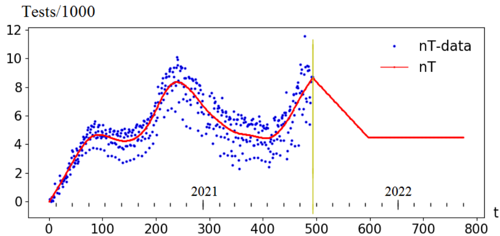
Fig. 11. Number of tests per thousand: data fitting and preset control (to the right of the yellow line).
