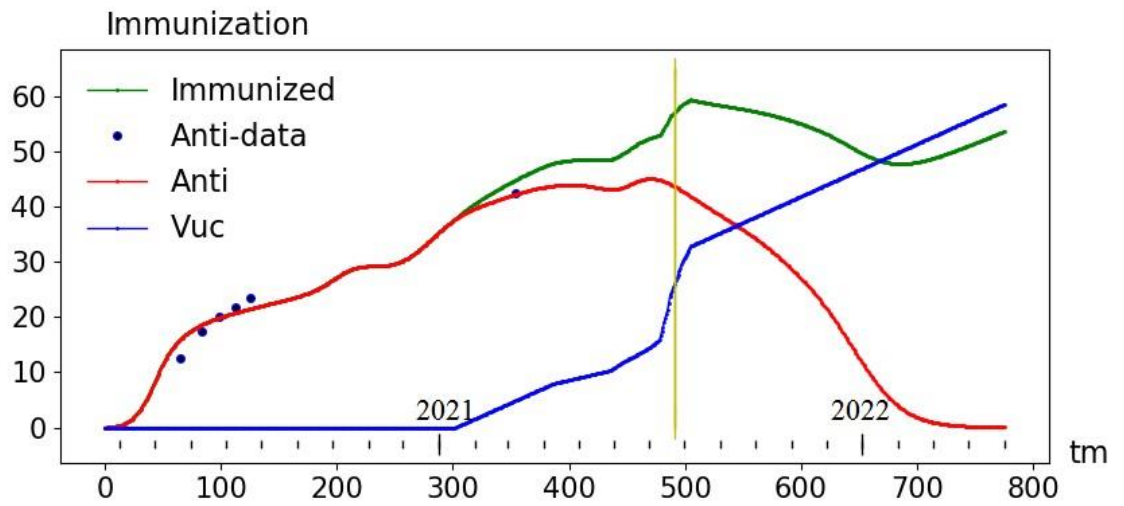
Fig. 8. Third wave forecast for Moscow from 25.07.2021.
