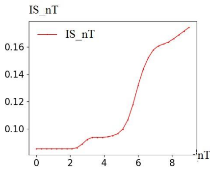
Fig. 2. IS_{nT} – a function of the effectiveness of detecting the infected depending on the number of tests per thousand ( nT ) in Moscow.
