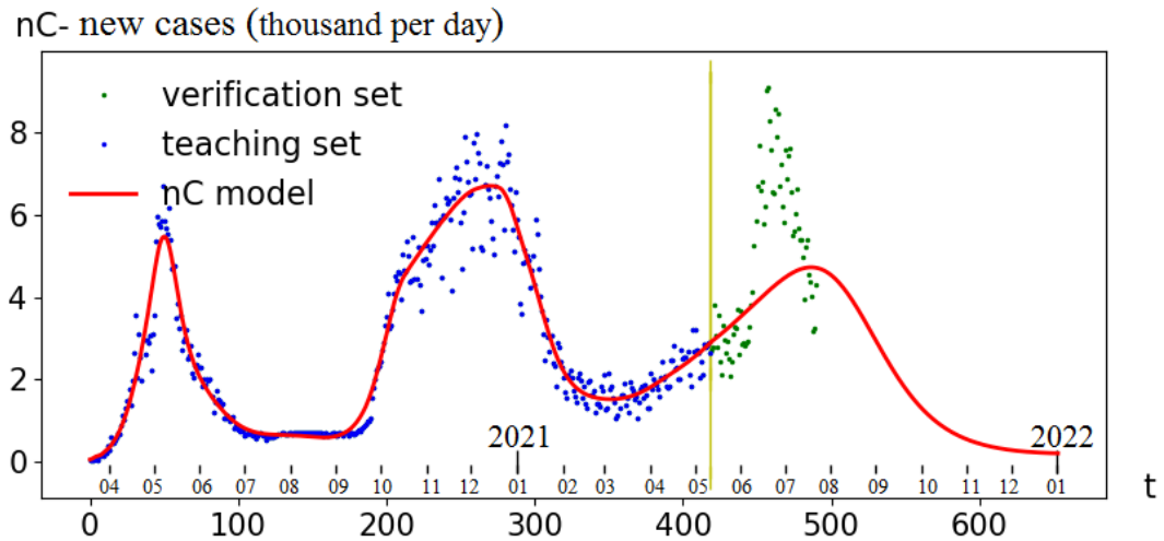
Fig. 7. Example of the third wave forecast for Moscow from 11.05.2021.
