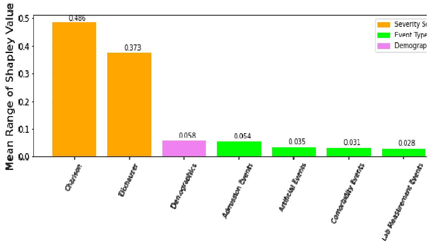
Figure 2. The Mean range of Shapley Values for each variable type
