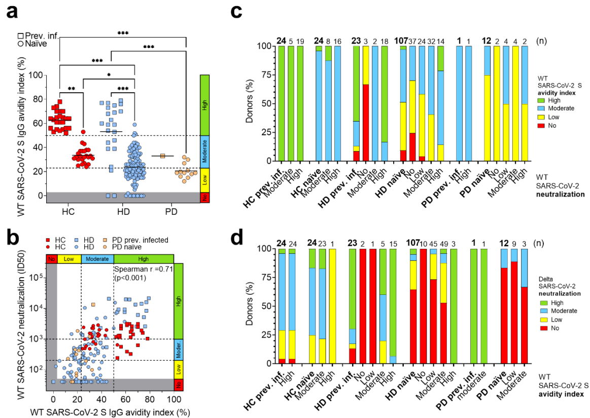
Figure 3 | Role of avidity of plasma antibodies in the neutralization of wild-type SARS-CoV-2 and Delta variant. (a) Avidity index of plasma antibodies to WT SARS-CoV-2 S in previously infected (square) and naïve (circle) healthy controls (HC), hemodialysis (HD) and peritoneal dialysis (PD) patients after two doses of mRNA vaccine. Grey areas indicate no avidity measured of plasma antibodies with ED50 titers lower than 50. A cut-off of 23%, determined from the lowest avidity index in naïve HC, and a cut-off of 50%, determined from the lowest avidity index in previously infected HC cohort, were used to distinguish low (0-23%) from moderate (23-50%) or high (>50%) avidity. Statistical significance is set as P < 0.05 and P-values are indicated with asterisks ( * = 0.033 ; ** = 0.002 ; *** < 0.001 ). Shown are data from n = 2 independent experiments. (b) Correlation analysis between plasma IgG avidity index to WT SARS-CoV-2 S and neutralization of WT SARS-CoV-2 in all the plasma samples collected after the second vaccine dose. (c) Percentages of donors having plasma antibodies with high, moderate, low or no avidity to WT SARS-CoV-2 S after two doses of mRNA
