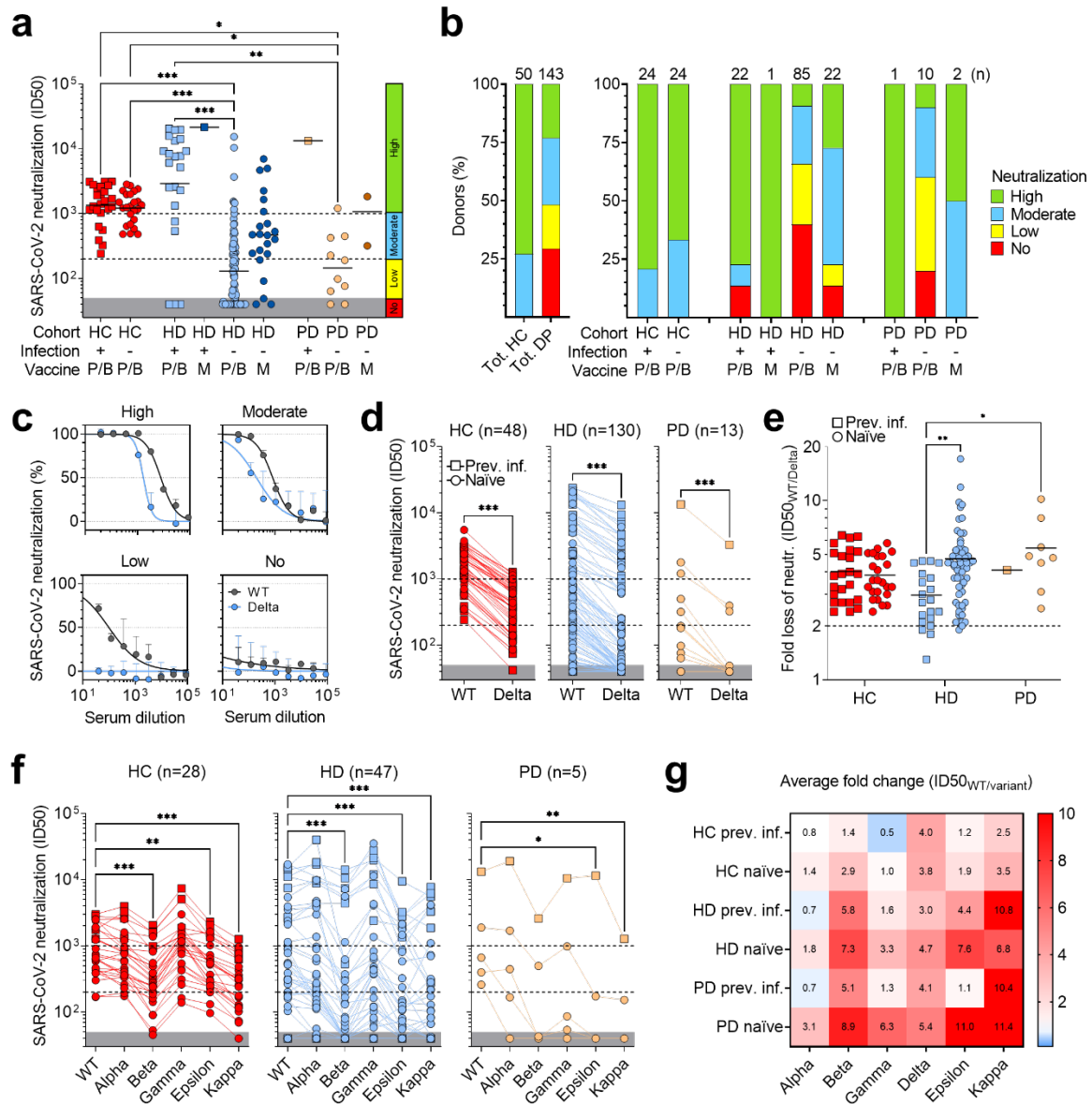
Figure 2 | Analysis of neutralizing activity of plasma antibodies against wild-type SARS-CoV-2, Delta and other variants. (a) Neutralizing antibody titers (ID50, 50% of inhibitory dilution) against pseudotyped VSV viruses harboring wild-type (D614) SARS-CoV-2 S determined using plasma from previously infected (square) and naïve (circle) healthy controls (HC), hemodialysis (HD) and peritoneal dialysis (PD) patients after two doses of Pfizer/BioNTech (P/B) or Moderna (M) vaccines. Grey areas indicate non-neutralizing titers (<50). A cut-off of 200, determined from the lowest neutralizing titers in HC, and a cut-off of 1'000, determined from the 25% percentile of titers in previously infected HC cohort, were
