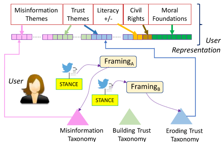
Figure 2: User representation for Profile Discovery.
