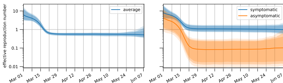
Figure 5: Temporal evolution of the effective reproduction number. The right plot shows the effective reproduction numbers for symptomatic and asymptomatic infected individuals, while the left plot shows their weighted average, i.e. the reproduction number for a generic infected individual. The bands correspond to 85%/90%/95% posterior credible intervals, while the solid line denotes the median value.
