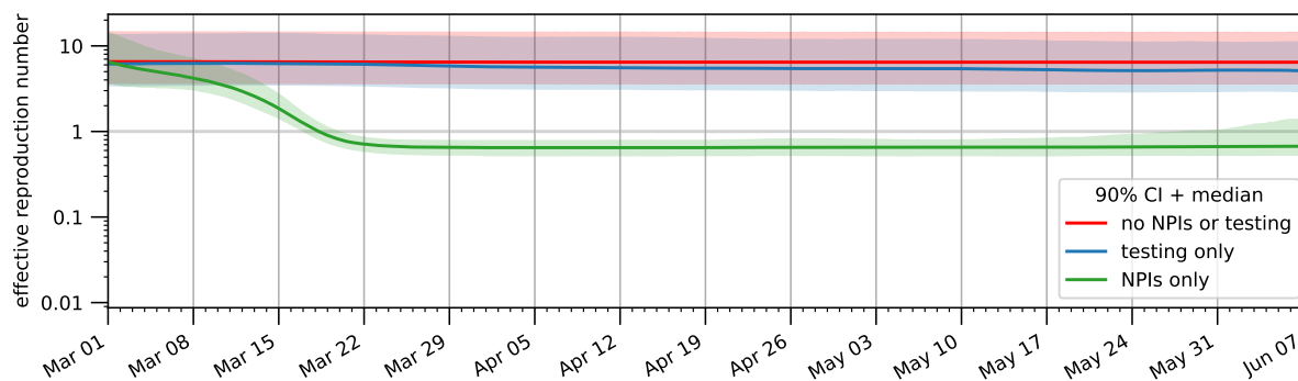
Figure 6: Relative importance of the detection process and the NPIs on the spread of the epidemic. Estimates for the reproduction number are plotted for three different scenarios: (red) neither diagnostic testing nor NPIs are employed; (blue) only diagnostic testing is performed; (green) only NPIs are applied. The bands correspond to the 90% posterior credible interval, while the solid line denotes the median value.
