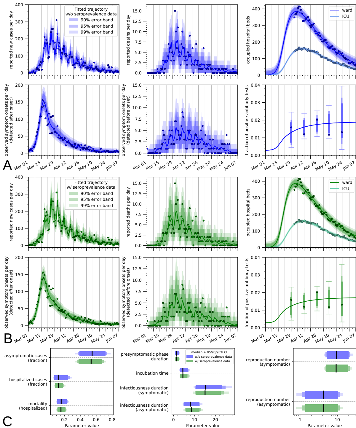
Figure 2: Modelling and parameter estimation for Munich, Germany. (A, B) Model simulation for the sampled parameter vector with the highest posterior probability compared with the observed data. In (A) only the case numbers reported by the Robert-Koch Institute and hospital usage for Munich are used for fitting, while in (B) seroprevalence data is also employed. The error bands show the range of plausible values for the observation, confirming that the noise models used are appropriate. In the bottom-right panels of (A, B), where the seroprevalence predicted by the model is plotted, the error bars are only shown at the observation times since the variance of each observation is linked to the number of total antibody tests carried out in each sub-batch. (C) Credible intervals (bars) and median value (line) for a subset of the model parameters. By reproduction number we mean the basic reproduction number in absence of NPIs and diagnostic testing (see Materials & Methods for more details on its computation).
