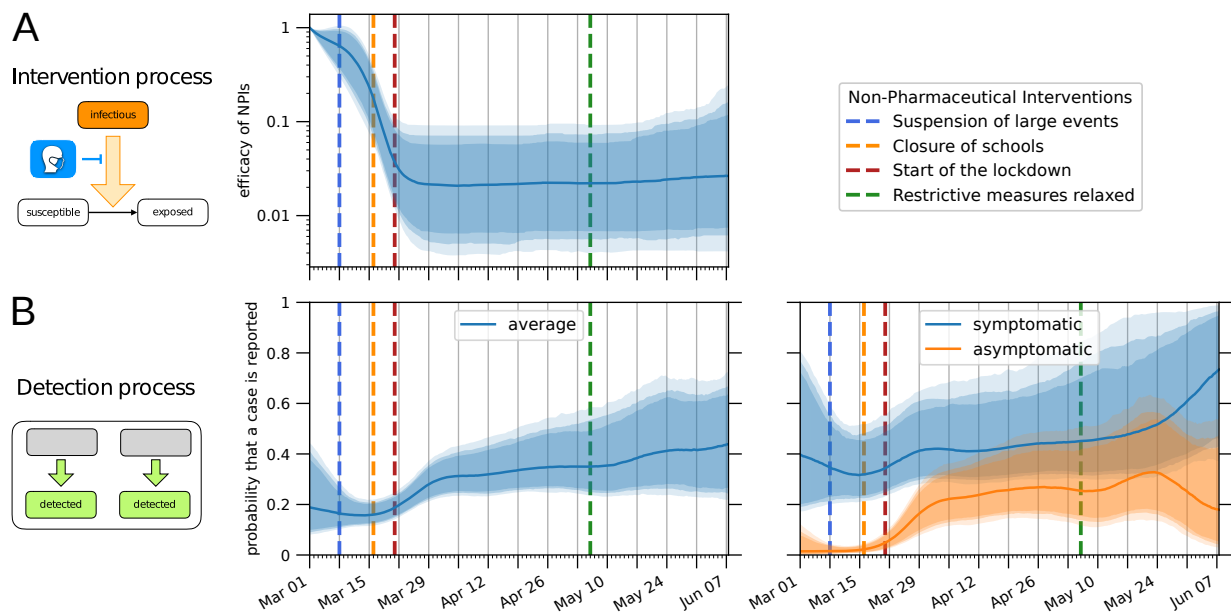
Figure 4: Estimation of time-dependent parameters. The bands correspond to 85%/90%/95% posterior credible intervals, while the solid line denotes the median value. Dashed lines indicate at which dates specific NPIs were enforced/lifted. (A) Reduction in the number of infectious contacts due to NPIs and behavioural changes, relative to the situation on March 1. (B) Probability that an infected individual is detected and reported to the healthcare authorities before the virus is cleared from their system. The left plot shows the average value, while the right plot shows separately the contributions due to symptomatic and asymptomatic individuals respectively.
