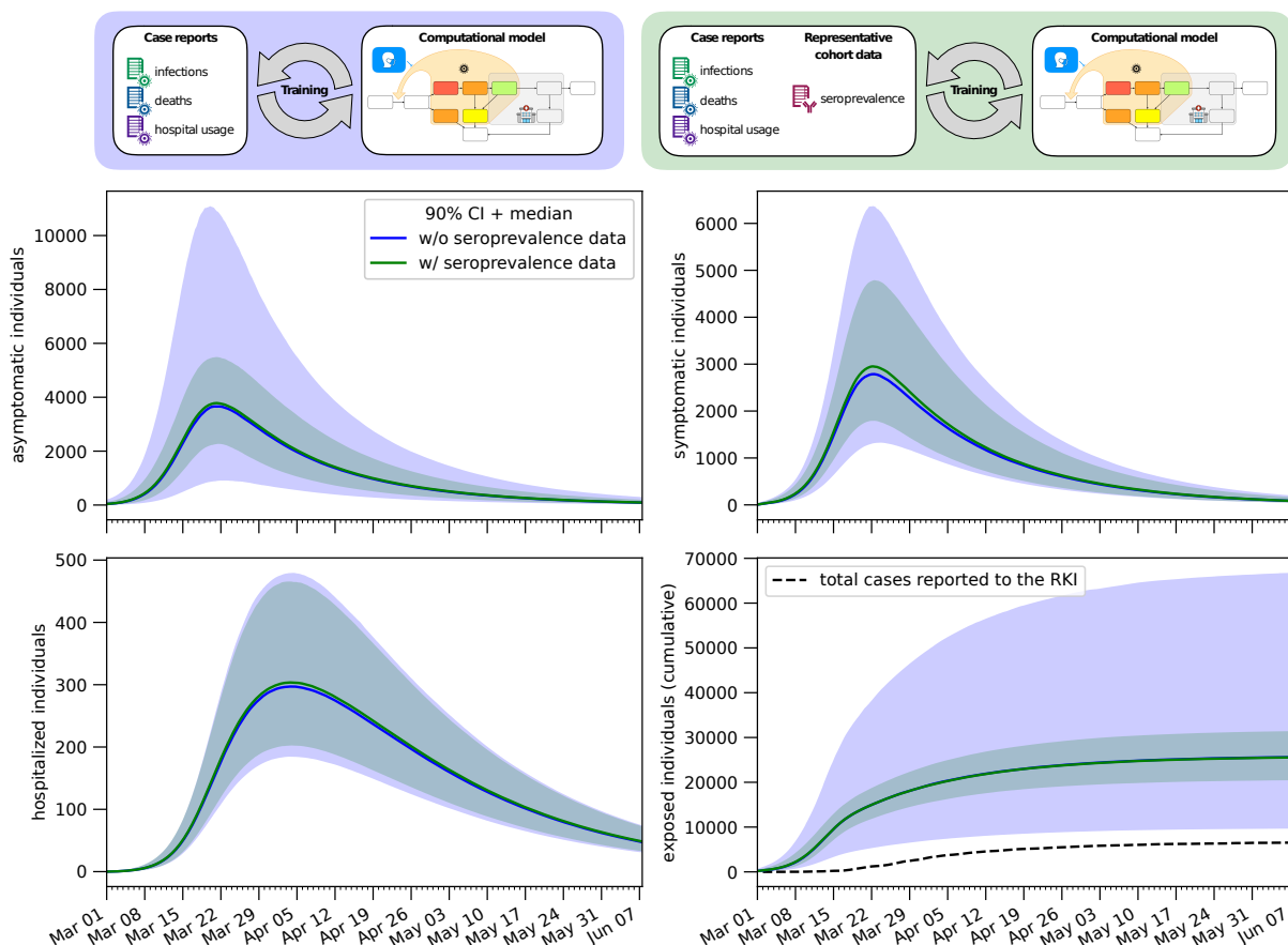
Figure 3: Estimates for the hidden dynamics of the epidemic. The number of individuals in different compartments is plotted as a function of time for both the model fitted with seroprevalence data and the one fitted without. In the bottom-right panel the cumulative number of cases detected by the healthcare authorities is also plotted for reference. The bands correspond to 90% posterior credible intervals, while the solid line denotes the median value.
