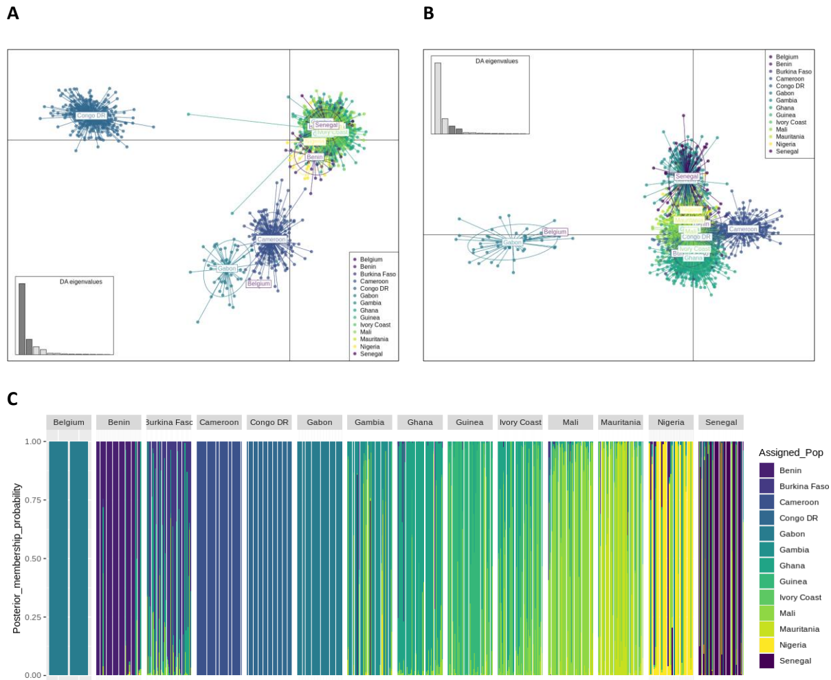
Figure 2. Discriminant analysis of principle components (DAPC). A) Scatter plot of DA eigenvalues 1 and 2, positioning Belgian isolates with Cameroon and Gabon; B) Scatter plot of DA eigenvalues 3 and 4, positioning Belgian isolates with Gabon; C) Composition plot of predicted posterior membership probability for Belgian isolates using DAPC with all Western and Central African isolates.
