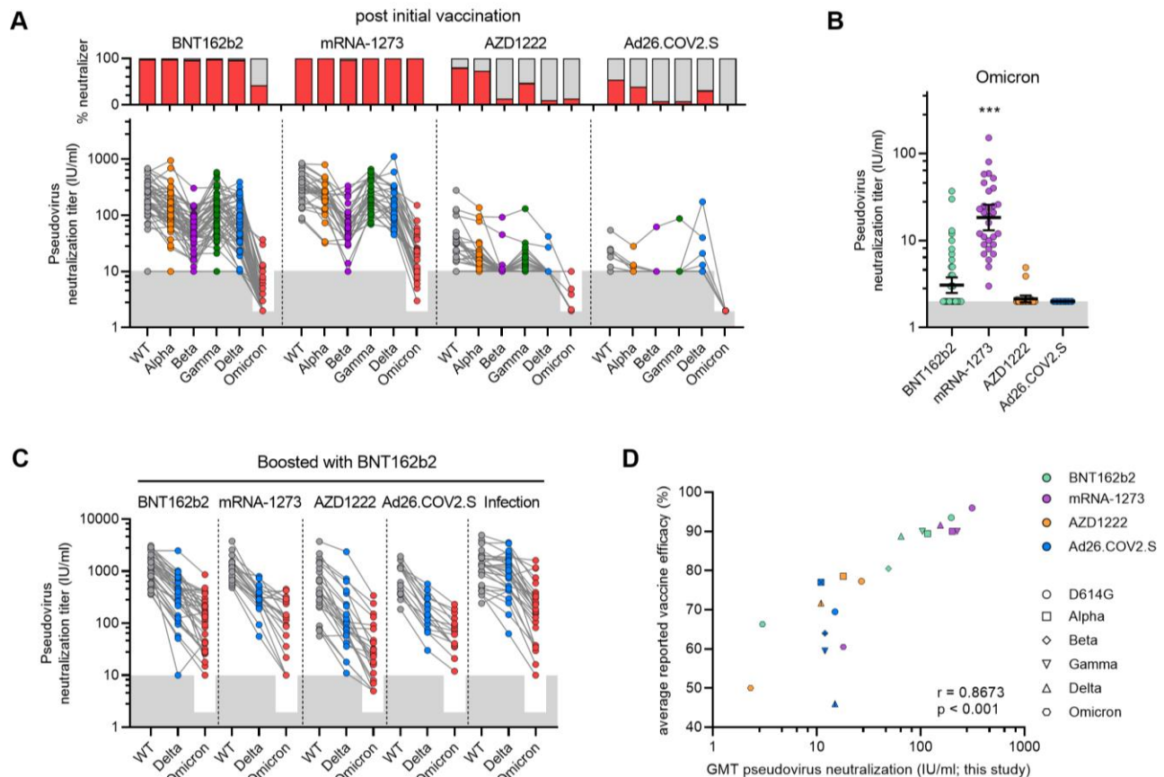
Figure 2: Binding and neutralization titers post-vaccination against VOCs. (A) Paired neutralization IC 50 titers (IU/ml) of D614G and VOCs pseudoviruses for sera collected post initial vaccination series for the four vaccination groups (lower panel). The lower cut-off for neutralization was set at an IC 50 of 10 or for Omicron at 2 IU/ml (grey shading). Percentage vaccinee with detectable neutralization titers in red (upper panel). (B) Neutralization titers of Omicron pseudovirus for sera post initial vaccination series. Geometric mean titer (GMT) and 95% CI are indicated. The lower cutoff for neutralization was set at an IC 50 of 2 IU/ml (grey shading). *** p < 0.001 non-parametric Kruskal-Wallis test for mRNA-1273 compared to the other groups. (C) Paired neutralization IC 50 titers (IU/ml) of D614G and VOCs pseudoviruses for sera collected post booster vaccination for the four vaccination groups and convalescent group (RECoVERED cohort; four weeks after single dose BNT162b2 vaccination up to 15 months post infection, n=28 ). The lower cut-off for neutralization was set at an IC 50 of 10 or for Omicron at 2 IU/ml (grey shading). Uni- and multivariable linear regression analysis results in Table S4. (D) GMT IC 50 neutralization titers of D614G and VOCs plotted against the average of reported vaccine efficacy against symptomatic infection (Table S2). Vaccine groups are indicated by colors with BNT162b2 in green, mRNA-1273 in purple, AZD1222 in orange and Ad26.COVS.2 in blue. Circles represent WT data, squares for Alpha, diamond for Beta, nabla triangle for Gamma and delta triangle for Delta. Crossed symbols are at the neutralization cutoff. Spearman's rank correlation coefficient with p -value are indicated.
