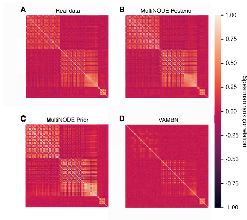
Figure 3: Correlation structure of real and synthetic data expressed as spearman rank correlation coefficients. Equivalent results for the NACC data are shown in Figure S6 . A , real data. B , posterior sampling from MultiNODEs. C , prior sampling from MultiNODEs. D , VAMBN generated data.
