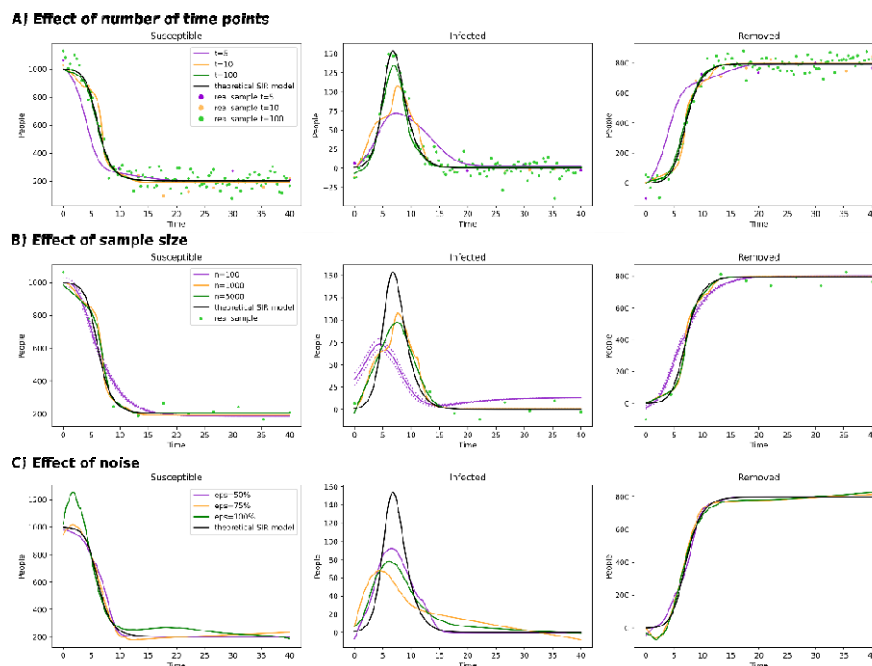
Figure 6: Model benchmarking on simulated data from the SIR-model. Each row represents the evaluation of another parameter (assessment frequency, sample size, noise level).
