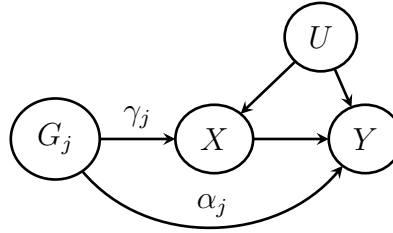
Figure 1: The relationships among the j th genetic variant G_j , the exposure X , the outcome Y and the unmeasured confounder U . The effect of G_j on X is \gamma_j , the direct effect (pleiotropic effect) of G_j on Y is \alpha_j , and the causal effect of X on Y is \beta .
