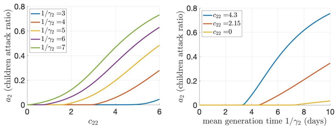
Figure 2: Attack ratio of COVID-19 among children ages 0-11 years in Ontario. The attack ratio depicted as a function of C_{22} (left panel) and 1/\gamma_2 (right panel) for different values of 1/\gamma_2 (left panel) and C_{22} (right panel) when 1/\gamma_1 = 3 and C_{11} = 10 .
