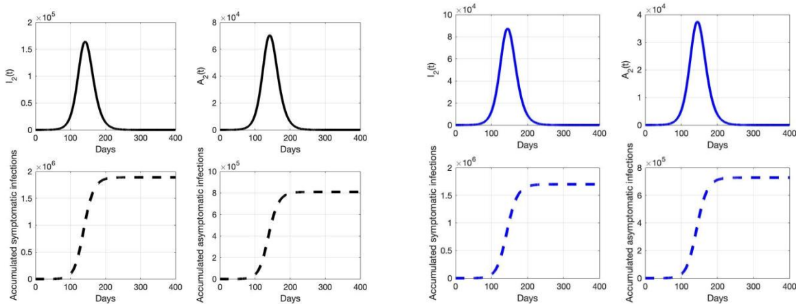
Figure B4: Canada epidemic curves , among children ages 0-11 years when C_{22} = 2.235 , C_{11}=10 , 1/\gamma_1 = 7 , for different values of 1/\gamma_2 (left panel in black color for 5 days, and right panel in blue color for 3 days). Initial infections for the vaccine-eligible are 100 and 10 for children.
