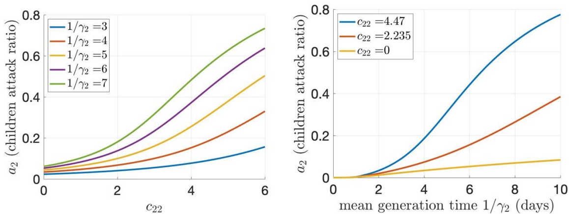
Figure B1: Canada attack ratio among children ages 0-11 years as a function of C_{22} (left panel) and 1/\gamma_2 (right panel) for different values of 1/\gamma_2 (left panel) and C_{22} (right panel) when 1/\gamma_1 = 3 and C_{11} = 11.27 .
