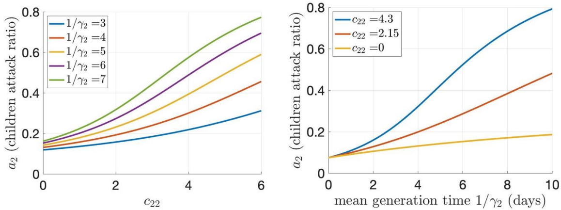
Figure 3: Attack ratio of COVID-19 among children ages 0-11 years. The attack ratio is assessed as a function of C_{22} (left panel) and 1/\gamma_2 (right panel) for different values of 1/\gamma_2 (left panel) and C_{22} (right panel) when 1/\gamma_1 = 4 and C_{11} = 10 .
