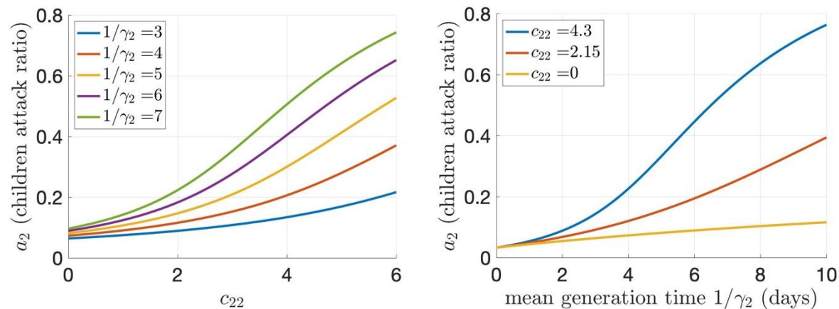
Figure 1: Attack ratio of COVID-19 among children ages 0-11 years in Ontario. The attack ratio is depicted as a function of C_{22} (left panel) and 1/\gamma_2 (right panel) for different values of 1/\gamma_2 (left panel) and C_{22} (right panel) when 1/\gamma_1 = 3 and C_{11} = 12.73 .
