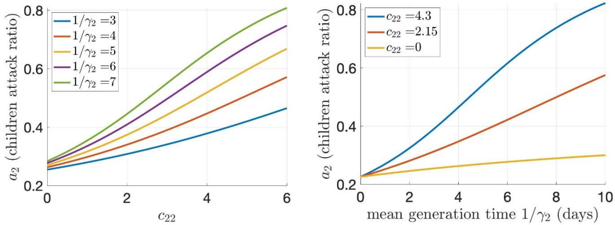
Figure 4: Attack ratio of COVID-19 among children ages 0-11 years in Ontario. The attack ratio is shown as function of C_{22} (left panel) and 1/\gamma_2 (right panel) for different values of 1/\gamma_2 (left panel) and C_{22} (right panel) when 1/\gamma_1 = 5 and C_{11} = 10 .
