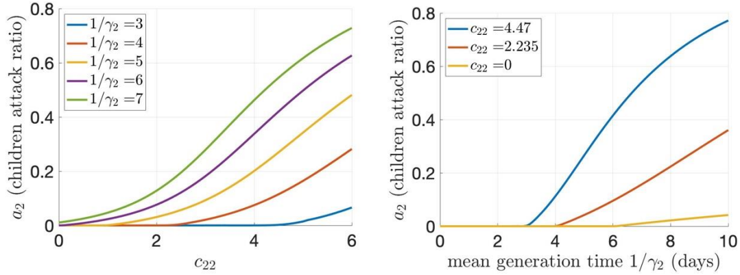
Figure B2: Canada attack ratio among children 0-11 years as a function of C_{22} (left panel) and 1/\gamma_2 (right panel) for different values of 1/\gamma_2 (left panel) and C_{22} (right panel) when 1/\gamma_1 = 3 and C_{11} = 10 .
